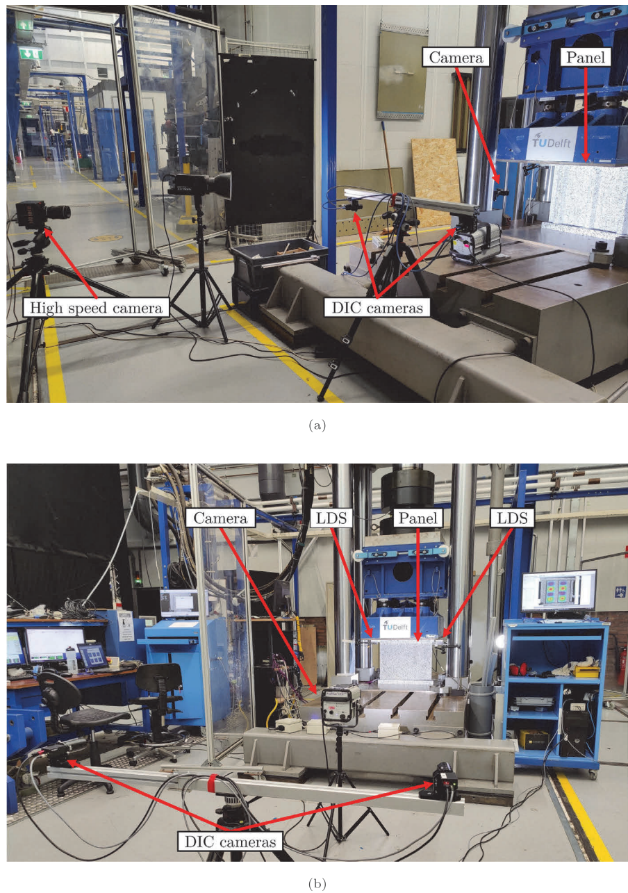
Fig. 11. Test setup seen from: (a) stringer side; (b) skin side.
