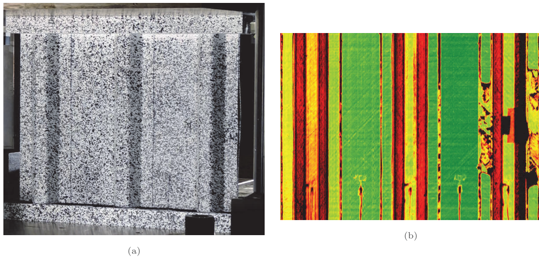
Fig. 38. Post-failure of panel 4: (a) photo; (b) c-scan.
