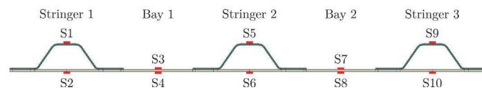
Fig. 4. Strain gauge locations.
