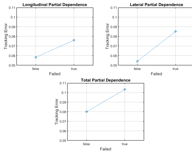
Figure 27: Partial Dependence of Failure.
