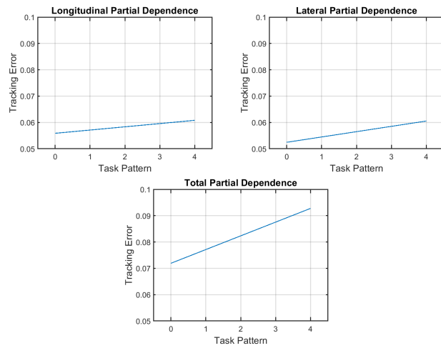
Figure 26: Partial Dependence of Task Patterns.
