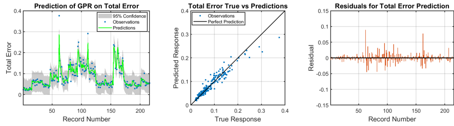
Figure 23: Gaussian Process Regression for total data.
