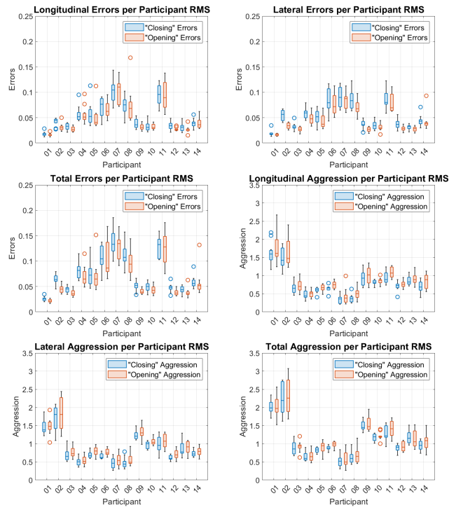
Figure 13: Error and Aggression RMS under the Closing and Opening conditions.
