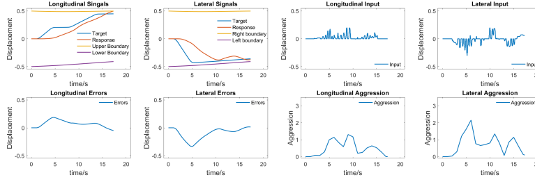
Figure 19: Task failed while ignoring one axis.
