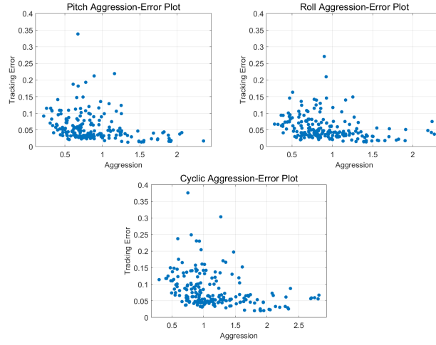
Figure 20: Aggression-Error plot.
