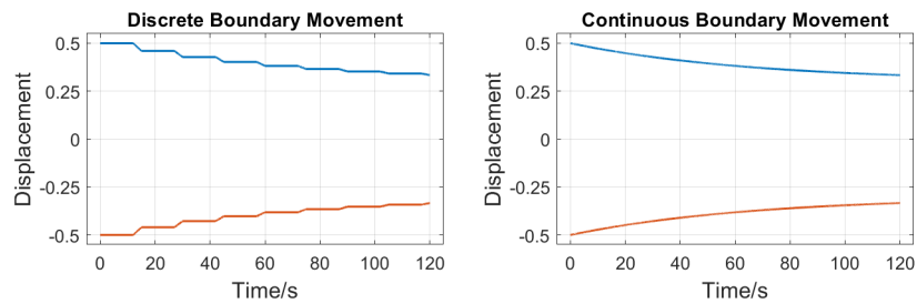
Figure 6: “Discrete” and “continuous” boundary movement.
