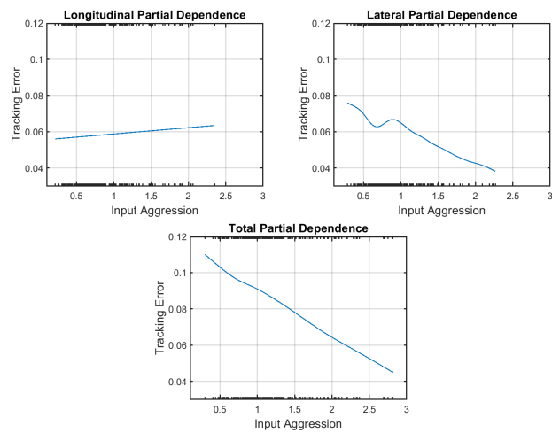
Figure 28: Partial Dependence of Aggression.
