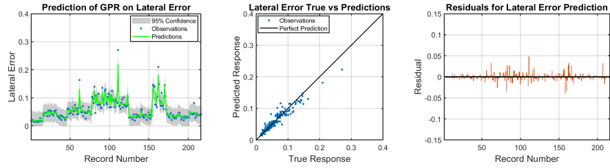
Figure 22: Gaussian Process Regression in the Lateral Axis.
