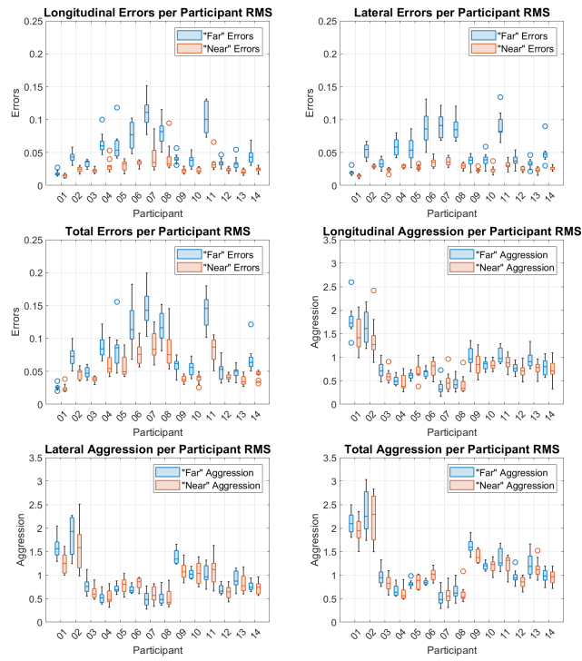
Figure 14: Error and Aggression under the Near and Far conditions.
