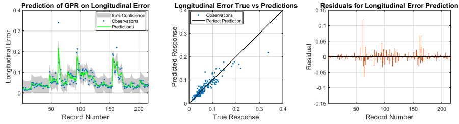
Figure 21: Gaussian Process Regression in the Longitudinal Axis.
