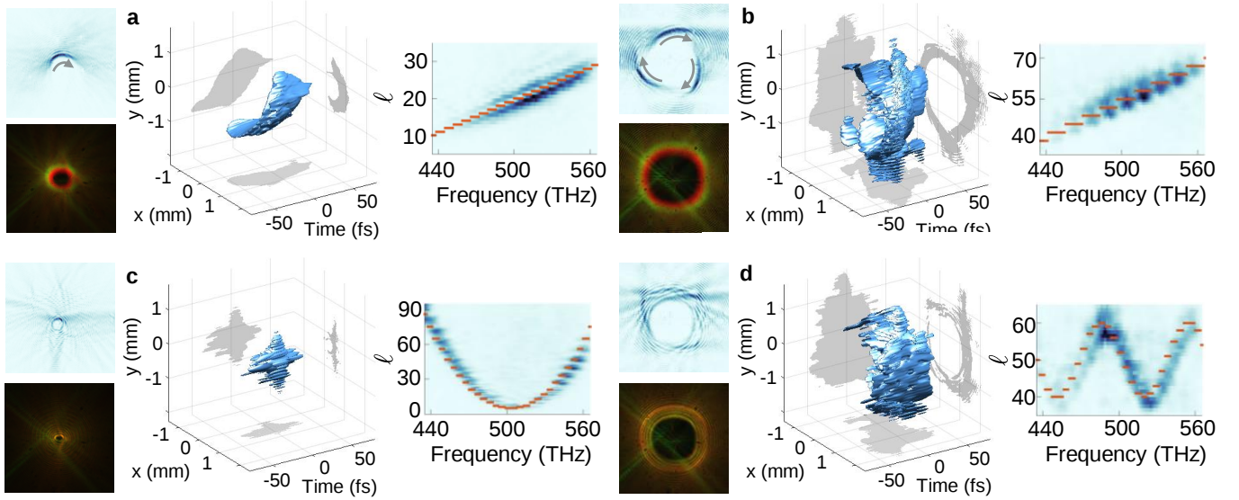
Extended Data Fig. 2. Additional linear and complex topological-spectral correlations. a , Linear correlation with OAM spanning from \ell = 10 to 30 corresponding to a helical wave packet with small orbital radius. b , Three intertwined helices obtained by employing discrete steps with \delta\ell = 3 in the correlation. c , Parabolic correlation with broadband OAM content spanning from \ell = 5 to 90 . d , Sinusoidal correlation completing two full oscillations over the spectral bandwidth. Due to the symmetry of the sinusoidal function, the reconstructed intensity does not show oscillations, analogously to the achiral wave packet obtained from parabolic correlations in Fig. 4d. Each panel shows the intensity of the electric field at t = 0 (top left), the time-averaged color image of the beam obtained by an hyperspectral camera (bottom left), the iso-surface at 10% of the intensity peak (center), and the experimental correlation (right). The size of the intensity and color images is 4 mm.
