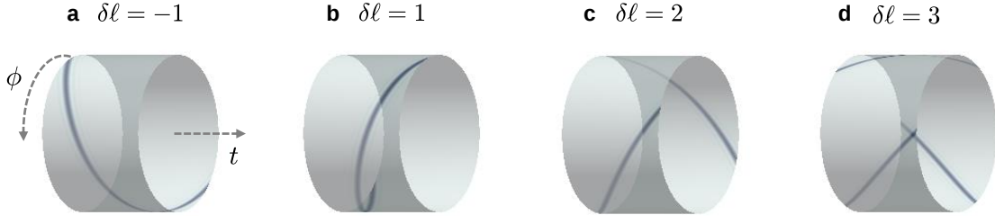
Extended Data Fig. 3. Chirality and number of intertwined helices obtained from the analytical theory. \delta\ell is a parameter in our analytical theory of helical wave packets with linear topological-spectral correlations corresponding to the discrete step in OAM value between two neighboring spectral windows. Cylinders represent the 2D space defined by the azimuthal angle and time variable, and on their surfaces we plot the intensity of the wave packet from Eq. S12 of Supplementary Note 7. a,b , By changing the sign of \delta\ell , the chirality of the helical wave packet changes. b–d By increasing the magnitude of \delta\ell , the number of intertwined helices increases correspondingly.
