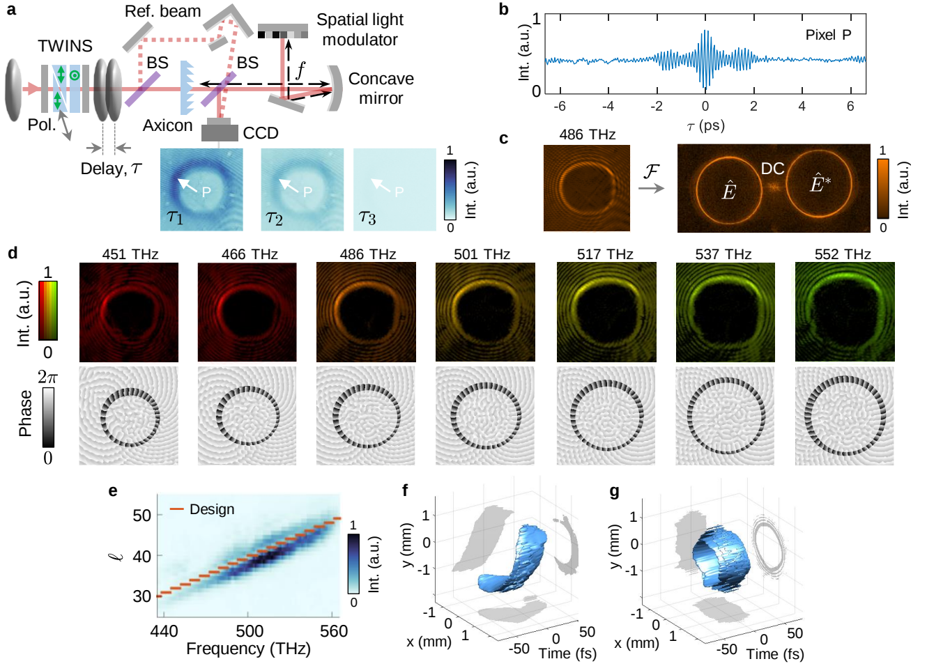
Fig. 2. Spatiotemporal characterization based on hyperspectral off-axis holography. a , Schematic of the spatially-resolved spectral setup introduced for the space-time beam characterization. It combines a spatial interferometer based on off-axis digital holography with a temporal one based on Fourier transform spectroscopy using a common-path birefringent interferometer, the Translating-Wedge-based Identical pulses eNcoding System (TWINS). Both the axicon and the SLM lie at the focal distance ( f ) of the concave mirror. Three images recorded by the CCD camera, which lies at the image plane ( 4f ) of the axicon, show the change in signal intensity at different delays \tau of the TWINS interferometer, ranging from constructive ( \tau_1 ) to destructive interference ( \tau_3 ). BS, beamsplitter. b , Interferogram signal at the pixel P marked in a . c , Off-axis interference image at 486 THz that, upon a digital spatial Fourier transform, gives the first-order complex conjugates of the electric field ( \hat{E} and \hat{E}^* ) and the non-interfering components (DC). d , Intensity and phase images of the complex electric field obtained after the off-axis digital holography analysis and shown for a selected set of frequencies from the hyperspectral cube. e , Experimental topological-spectral correlation of a helical wave packet obtained by modal decomposition. f,g , Iso-intensity surfaces at 10% of the intensity peak for the helical wave packet with the correlation shown in e and for a pulsed vortex with constant \bar{\ell} = 40 . The qualitative features of the iso-surfaces are independent from the specific percentage level chosen for the cut.
