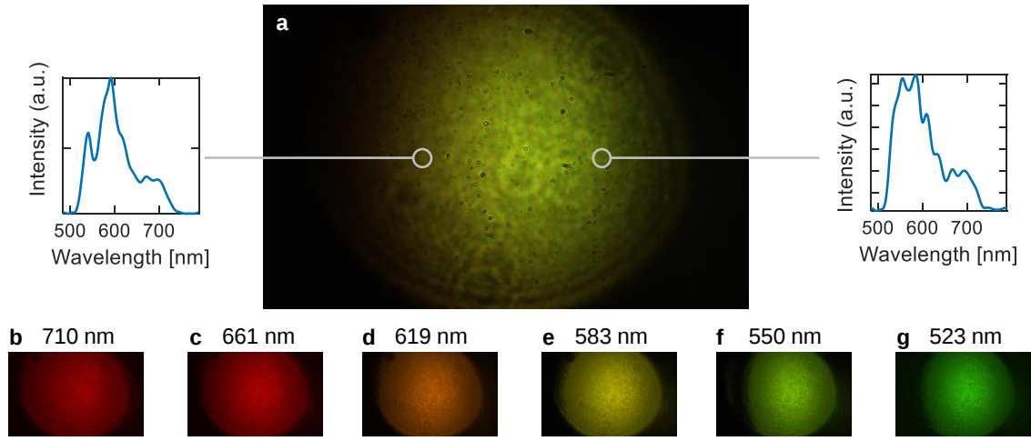
Extended Data Fig. 5. Spectrally-resolved beam profiler images of the NOPA beam measured with TWINS. a , RGB image of the NOPA beam at the output of the parametric amplifier. The spectrum measured on the left side of the beam has a weaker component in the green region as compared to the right side of the beam, corresponding to a small spatial chirp on the beam, in the sense that the spatial intensity profile has a slight frequency dependence . b–g , Spectral images of the beam for a selected set of wavelengths ranging from 710 nm to 523 nm obtained using the hyperspectral measurement technique. The size of all images is 11.2 mm \times 7.0 mm.
