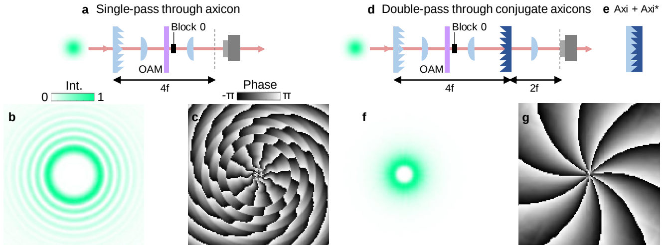
Extended Data Fig. 6. Generation of OAM-carrying Bessel-Gauss or Laguerre-Gauss beams by a single or double pass through axicons in our system. The numerical simulations assume an input Gaussian beam with 500 nm wavelength entering the setup. The phase plate imparting OAM in the far field of the axicon has a charge \ell = 10 . a , Setup schematic for OAM-carrying Bessel-Gauss beam generation. The detection plane (vertical dashed line) is slightly shifted from the 4f plane to allow for the formation of the Bessel-Gauss beam (as in Supplementary Fig. S4a). b,c , Simulated intensity and phase of the beam at the detection plane showing a Bessel-Gauss beam with \ell = 10 . d , Setup schematic for OAM-carrying Laguerre-Gauss beam generation. In this case a second negative axicon being the conjugate of the first positive axicon is placed at 4f . The detection plane is at 2f from the second axicon. e , Due to their complementary grating shapes, the phase contributions of the two axicons cancel out in this arrangement. f,g , Simulated intensity and phase of the beam at the detection plane showing a Laguerre-Gauss beam with \ell = 10 . In a and d the 4f imaging systems are shown unfolded for clarity and using lenses, though they can be implemented with a single spherical mirror as in Fig. 2a. An amplitude mask is used to block the zero order in the far field of the axicon.
