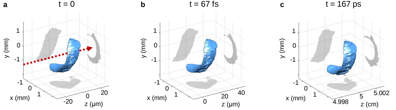
Extended Data Fig. 1. Isosurfaces in 3D space of a helical wave packet synthesized experimentally. The corresponding topological-spectral correlation of this beam is shown in Fig. 2e. Here, the temporal coordinate is replaced by the z -propagation coordinate, as we obtain from hyperspectral off-axis holography the space-time beam propagation at different times: a , t = 0 ; b , t = 67 fs, corresponding to a beam propagation of 20 \mu\text{m} ; c , t = 167 ps, corresponding to a beam propagation of 5 cm. Apart from a very small lateral shift, the beam essentially translates along the z -axis as it propagates (in the direction marked by the red arrow in a ). Due to its helical structure, at a given z -plane the space-time beam appears as a pulse that rotates over time on a circular trajectory, as shown in the space-time isosurface of Fig. 2f. The isosurfaces are defined at 10% of the intensity peak.
