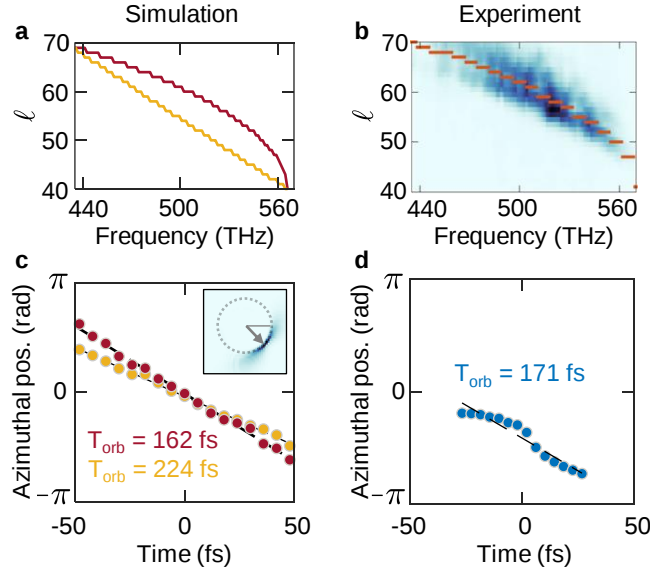
Extended Data Fig. 4. Simulated and measured orbital period of a wave packet synthesized from a square root correlation function. a , Correlations obtained from Eq. 1 using p = 0.5 (red) and, for comparison, p = 1 (yellow). The other parameters of the equation are \Delta\ell = 30 , \ell_1 = 40 , \Delta\omega/2\pi = 137 THz, \omega_2/2\pi = 566 THz. b , Experimental square root correlation function. c Azimuthal position of the maximum of the rotating pulse as a function of time obtained from the simulations using p = 0.5 (red) or p = 1 (yellow). By fitting the slopes corresponding to the angular velocity \Omega we obtain the orbital periods T_{\text{orb}} = 2\pi/\Omega reported in the plots, indicating that the complex correlation function produces a shorter T_{\text{orb}} and a larger \Omega . The inset shows how the azimuthal position is extracted at a given time from the maximum of the rotating space-time beam intensity. The simulation assumes a frequency chirp in the input beam equivalent to a group delay dispersion of 79 \text{ fs}^2 , as the one measured experimentally using hyperspectral holography. d Azimuthal position as a function of time obtained from the experimental space-time beam synthesized using the square root correlation function, giving a value close to the simulated one for p = 0.5 .
