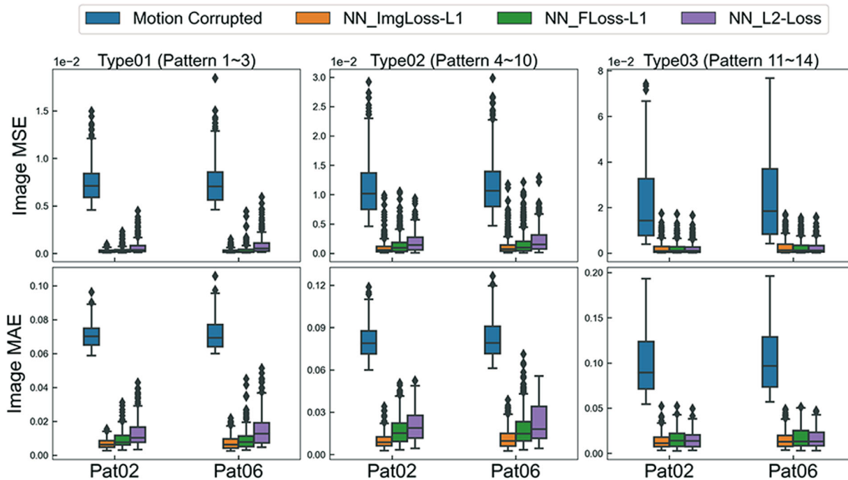
FIGURE 8 Box plots comparing the MSE (top) and MAE (bottom) for all the testing frames before and after intra-frame motion compensation. Testing frames are grouped by the type of intra-frame motion pattern. Note: all the images are normalized to [0, 1], and the y-axis has different scale limits among subfigures.
