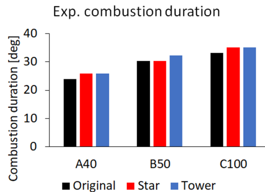
Figure 7. Comparison of the experimental combustion durations for the three operating points when using the three different piston bowls.
