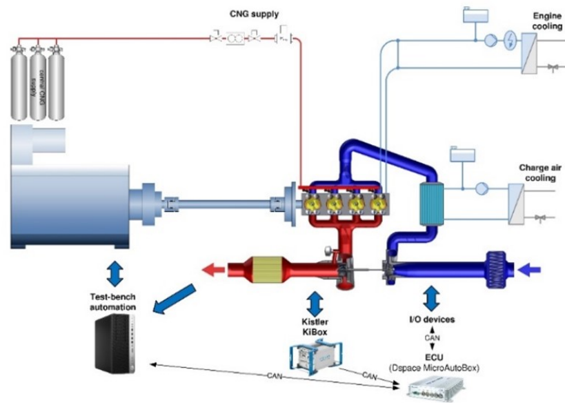
Figure 2. Test bench scheme.
