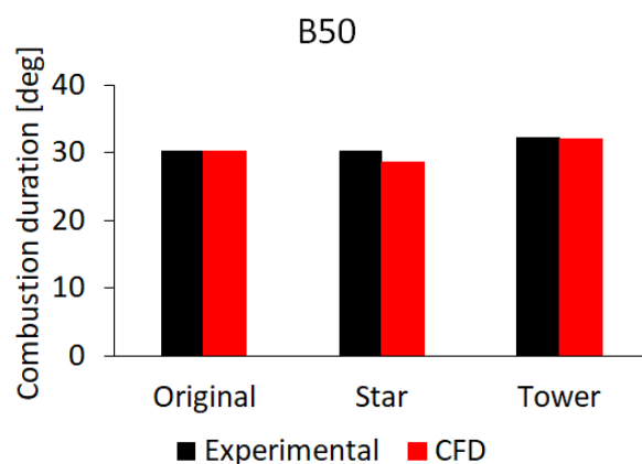
Figure 12. Comparison between the computed and experimental combustion durations for the B50 operating point and the three different piston bowls.
