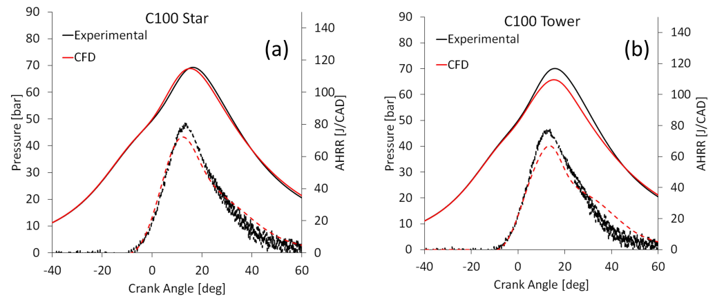
Figure 14. Comparison between the computed and experimental data of the in-cylinder pressure (solid lines) and apparent heat release rate (dashed lines) for the C100 operating point when using the star (a) and tower (b) pistons.
