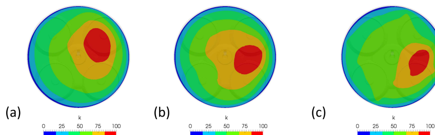
Figure 9. Kinetic energy distribution of turbulence on a plane orthogonal to the cylinder axis placed 5 mm below the cylinder head flow for the original (a), star (b), and tower (c) piston bowls.
