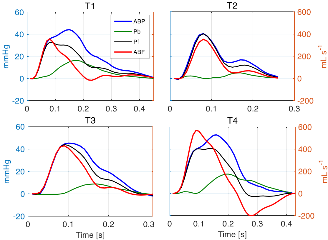
Fig. 8. Examples of forward (Pf, black line) and backward (Pb, green line) arterial blood pressure (ABP, blue line) waves computed in one septic pig at each time point of the experiment. All the signals are displayed so to start from 0 to highlight the amplitude ratios. ABF: arterial blood flow (red line); T1: baseline; T2: after sepsis development; T3: after 24 h of resuscitation; T4: after 48 h of resuscitation.
