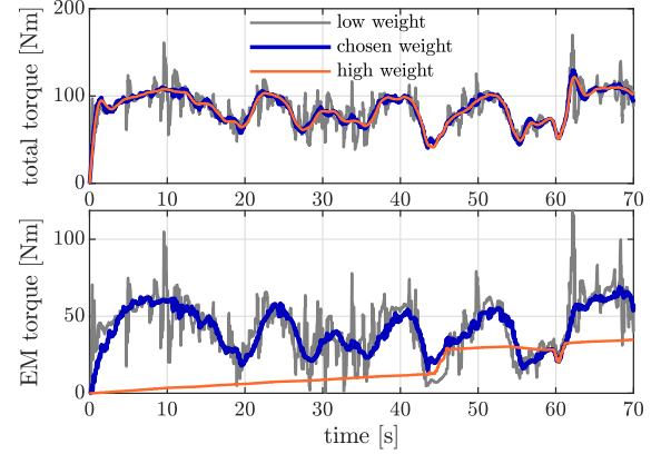
Fig. 13. Sensitivity w.r.t. the control weight c_{\text{control}} , in simulation environment.
