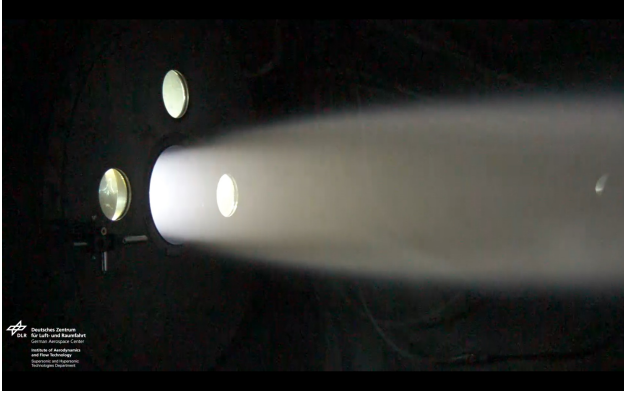
Figure 21: d_e = 200\text{ mm} , p_c = 0.59\text{ mbar}
