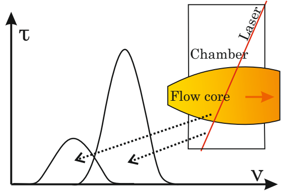
Figure 5: Expected absorption lines
