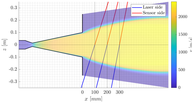
Figure 14: LOS interpolation tool
