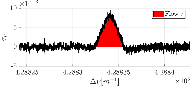
Figure 25: Absorption profile, p_c = 0.59 \text{ mbar}
