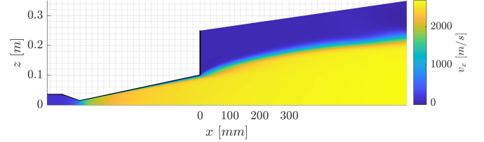
Figure 10: Axial velocity v_z
