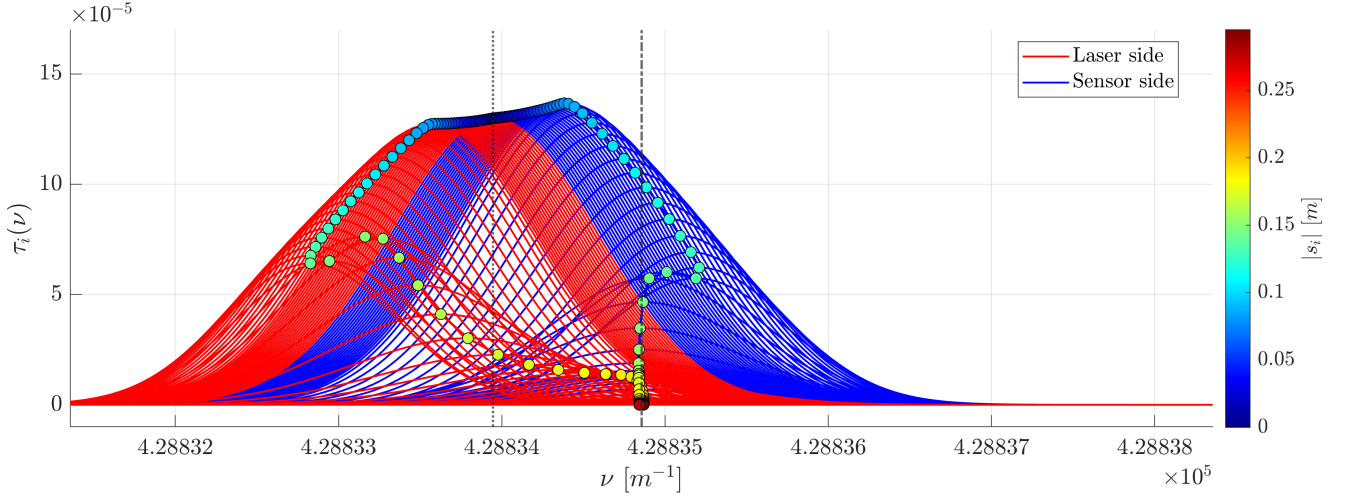
Figure 16: BLOB partial spectra, for measurement position x = 200 \text{ mm}
