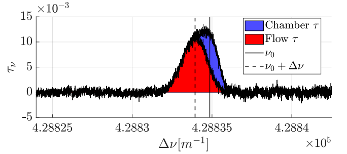
Figure 24: Absorption profile, p_c = 0.42\text{ mbar}
