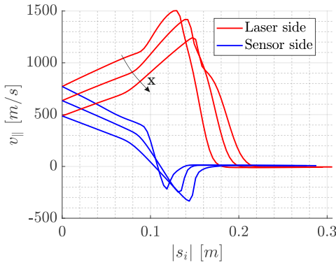
Figure 15: v_{\parallel} value, for all measurement positions
