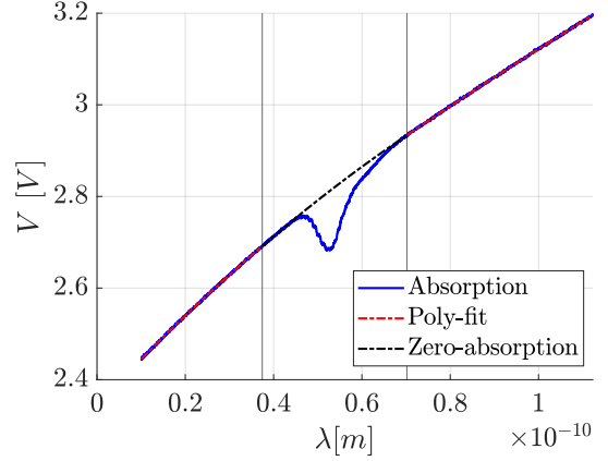
Figure 8: I_0 signal construction
