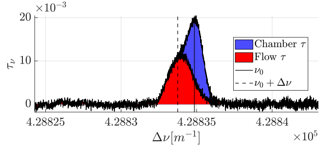
Figure 23: Absorption profile, p_c = 0.39\text{ mbar}
