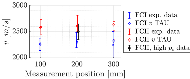
Figure 26: Flow axial velocity
