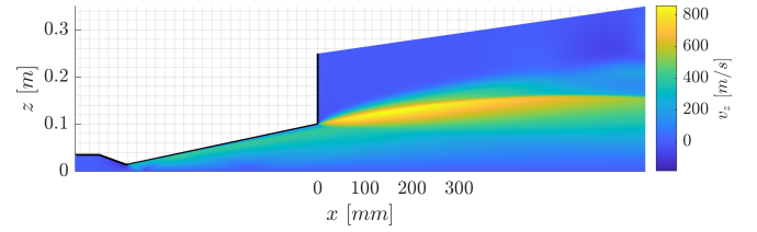
Figure 11: Radial velocity v_r
