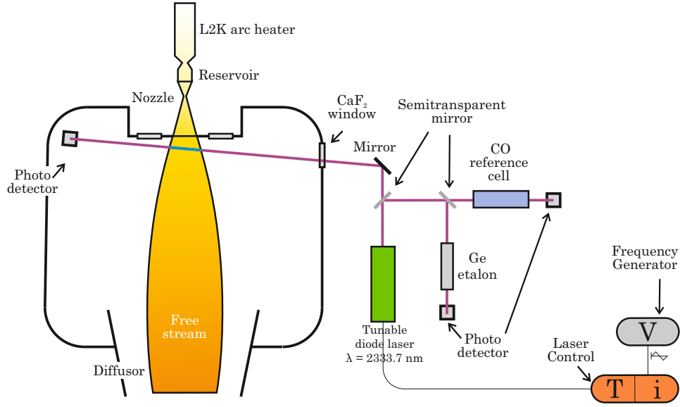
Figure 3: Conceptual scheme for TDLAS measurements
