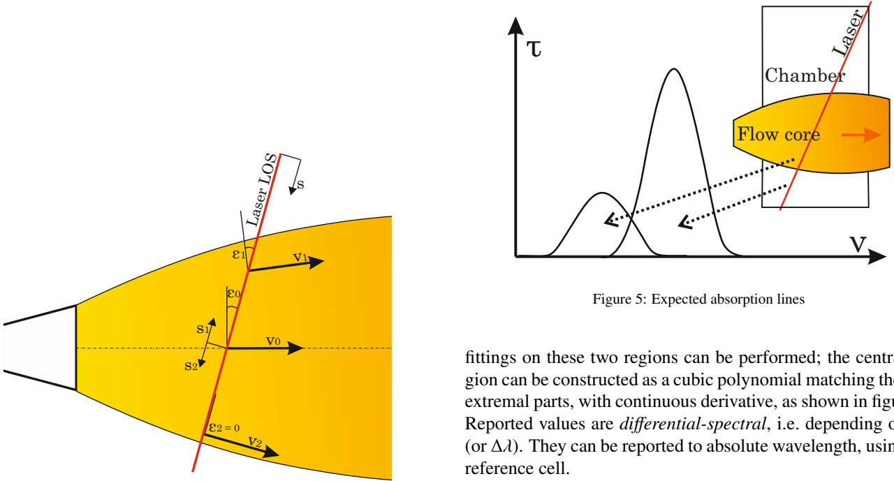
Figure 4: Flow geometry
