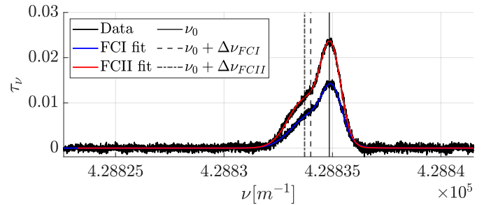
Figure 18: Measurement position x = 100 \text{ mm}
