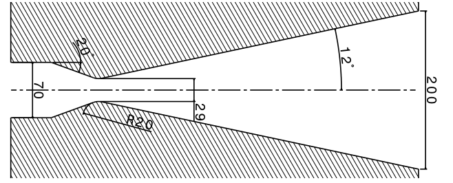
Figure 2: L2K nozzle geometry, 200 mm exit diameter configuration
