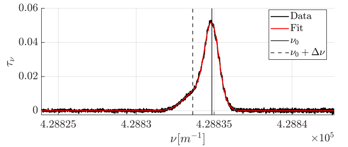
Figure 9: Optical depth, sweep 1
