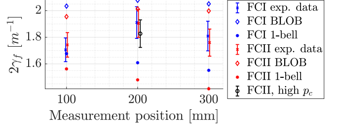
Figure 27: Line's FWHM
