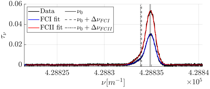
Figure 20: Measurement position x = 300mm
