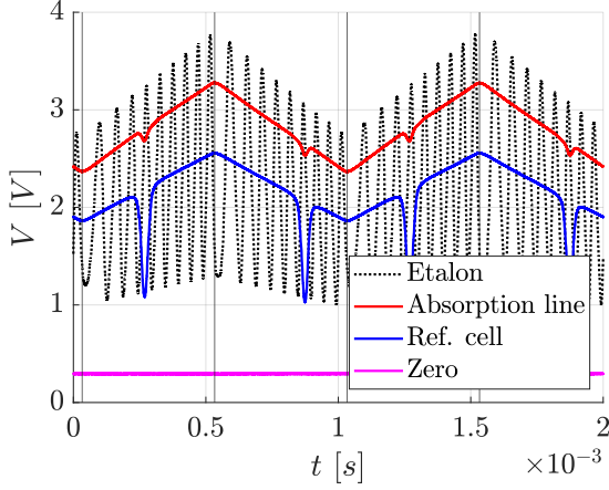
Figure 6: Raw oscilloscope data
