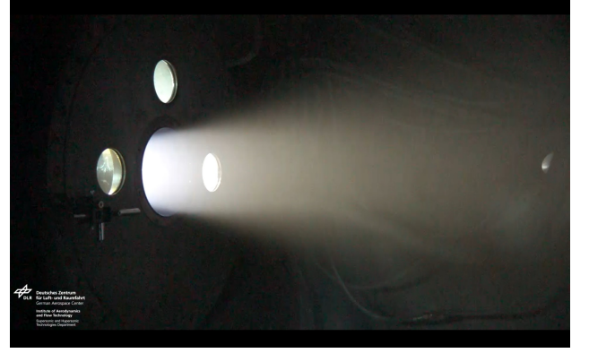
Figure 22: d_e = 200\text{ mm} , p_c = 0.07\text{ mbar}
