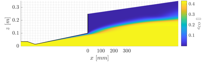
Figure 12: CO mass fraction
