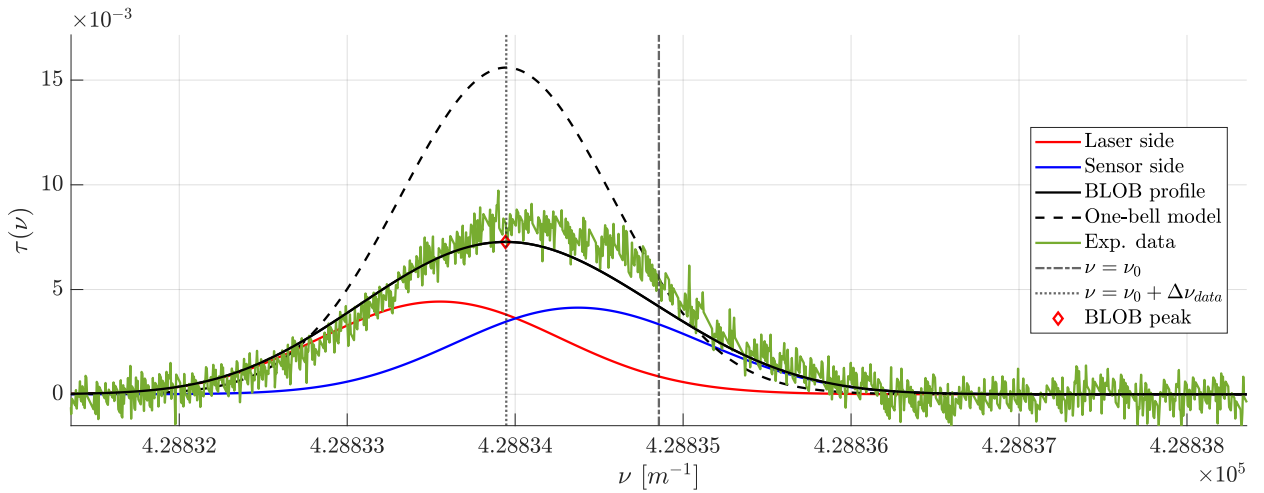
Figure 17: BLOB profile compared with experimental data, for measurement position x = 200 \text{ mm}
