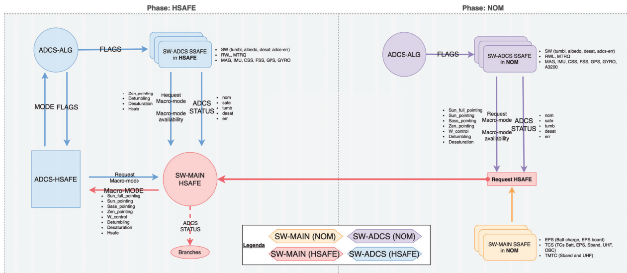
Figure 6: SW-ADCS NOM and HSAFE modes operational schemes.
