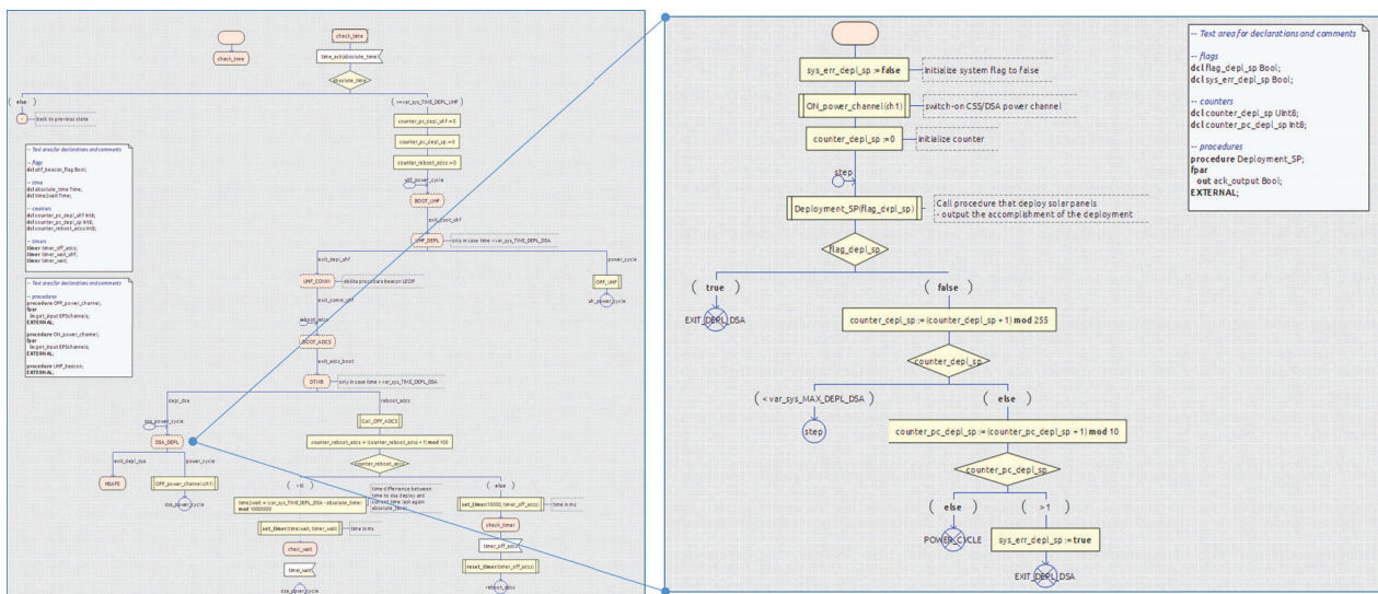
Figure 8: OpenGEODE implementation of the SW-MAIN LEOP mode, with a inside look at the Solar Array deployment state.
