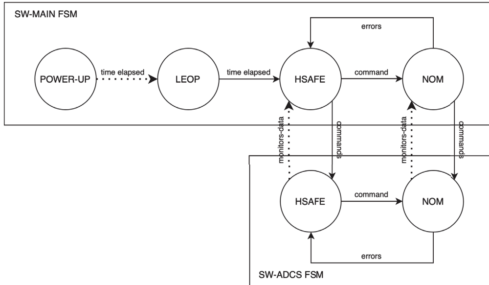
Figure 3: HERMES' software high-level structure.
