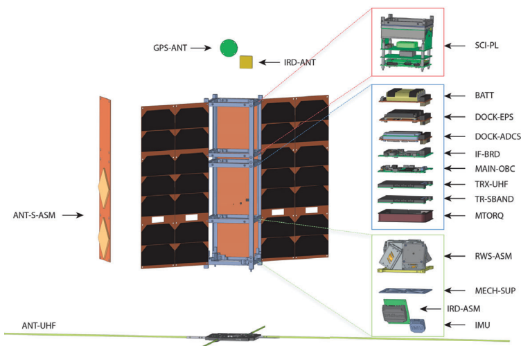
Figure 2: CAD description of the HERMES CubeSat's platform.
