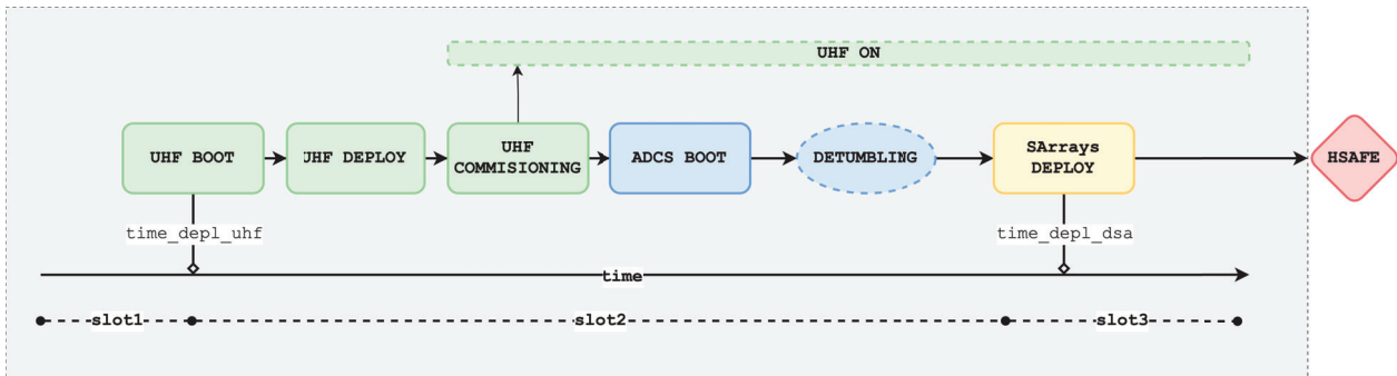
Figure 4: SW-MAIN LEOP mode operational schematic.
