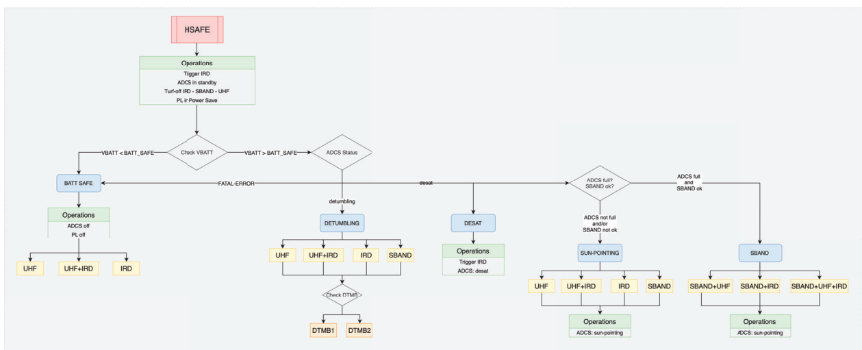
Figure 5: SW-MAIN HSAFE mode operational schematic.
