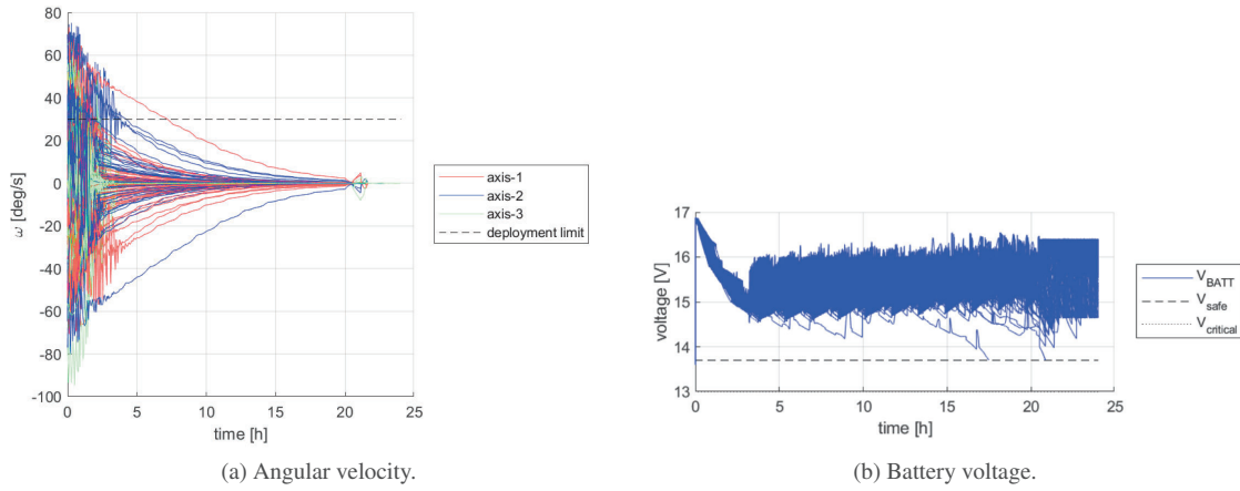
Figure 7: Montecarlo simulation during LEOP (50 runs).
