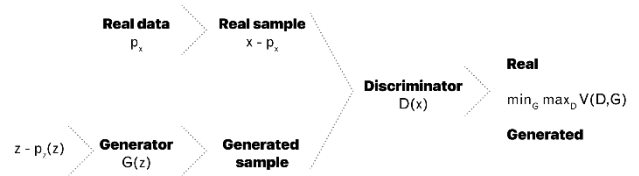
Figure 4: GAN functioning schema
