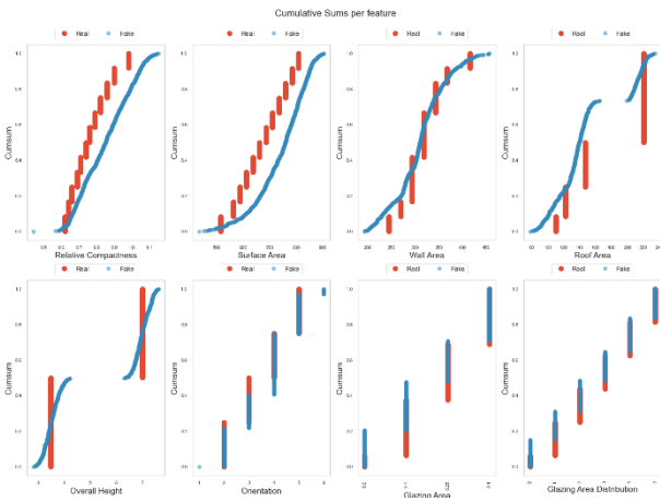
Figure 6: Real and synthetic data distribution for each feature
