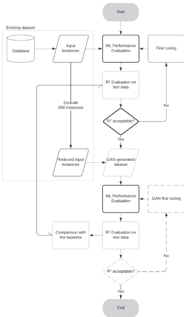
Figure 1: Methodology diagram
