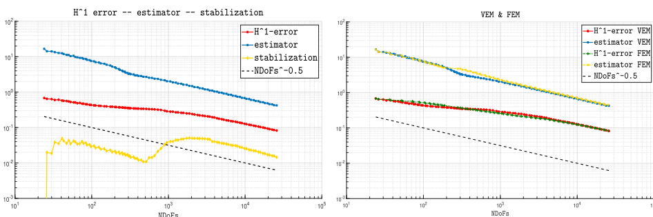
FIG 9. Test 2. Left: H^1 -error, estimator \eta_{\mathcal{T}}(u_{\mathcal{T}}, \mathcal{D}) , stabilization term S_{\mathcal{T}}(u_{\mathcal{T}}, u_{\mathcal{T}})^{1/2} . Right: H^1 -error and estimator \eta_{\mathcal{T}}(u_{\mathcal{T}}, \mathcal{D}) obtained with VEM and FEM. In both figures the optimal decay is indicated by the dashed line with slope -0.5 .
