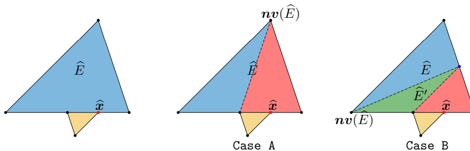
FIG 7. Left: mesh element \hat{E} having \hat{x} as a hanging node, with \hat{x} such that \lambda(\hat{x}) = \Lambda_{\mathcal{T}} > \Lambda . Middle, Case A: the node \hat{x} belongs to the opposite edge to the newest vertex of \hat{E} , therefore one bisection is needed. Right, Case B: the node \hat{x} belongs to the same edge of the newest vertex of \hat{E} , therefore two bisections are needed.
