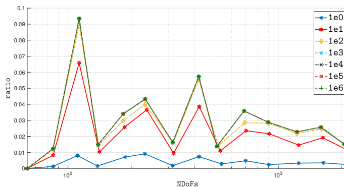
FIG 8. Test 1. Sharpness of bound (4.10): ratio between the term \gamma^2 S_{\mathcal{T}}(u_{\mathcal{T}}, u_{\mathcal{T}}) and the term \eta_{\mathcal{T}}^2(u_{\mathcal{T}}, \mathcal{D}) obtained with the adaptive algorithm (5.3).
