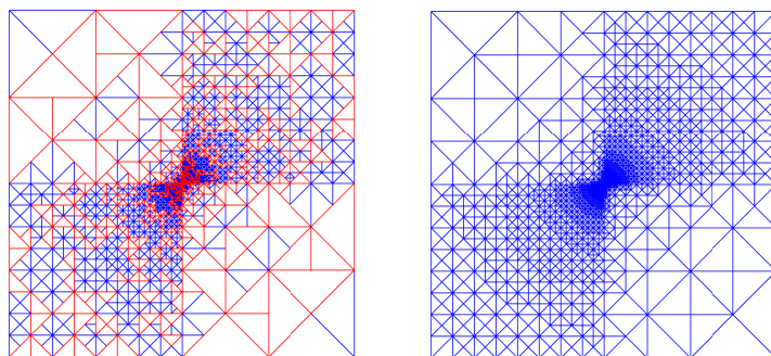
FIG 10. Test 2. Left: final grid \mathcal{T}_{\text{VEM}} obtained with VEM. Right: final grid \mathcal{T}_{\text{FEM}} obtained with FEM. Mesh elements having more than three vertices are drawn in red.
