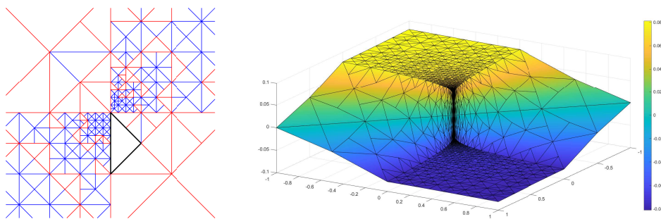
FIG 12. Test 2. Left: final grid \mathcal{T}_{\text{VEM}} , zoom to (-10^{-10}, 10^{-10})^2 (mesh elements having more than three vertices are drawn in red, and the mesh element drawn in black is a nonagon). Right: graph of the discrete solution.
