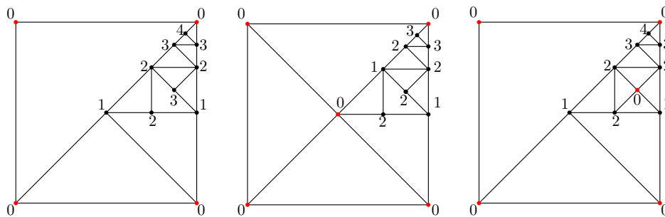
FIG 1. Three examples of distributions of proper nodes (red) and hanging nodes (black), with associated global indices \lambda . The bisection added in the middle picture converts the centered node into a proper node and induces nonlocal changes of global indices on chains associated with it. If \Lambda = 3 , then the leftmost mesh is not admissible and this procedure is instrumental to restore admissibility. The right picture illustrates the creation of a proper node without nonlocal effects on global indices.
