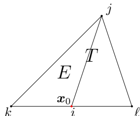
FIG 3. Sample of element E \in \mathcal{T} , where T = A(E) is the parent of E ; i, j, k are the global indices of the vertices of E ( i being the global index of \mathbf{x}_0 ); and \ell is global index of the remaining vertex of T .
