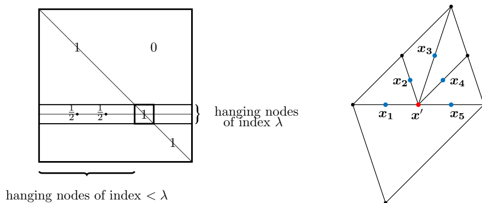
FIG 6. Left: structure of one factor \mathbf{W}_\lambda in the factorization (7.11). Right: given a hanging node \mathbf{x}' with \lambda(\mathbf{x}') < \lambda , at most five hanging nodes \mathbf{x}_i for i = 1, \dots, 5 of index \lambda may be such that \mathbf{x}' \in B(\mathbf{x}_i) .
