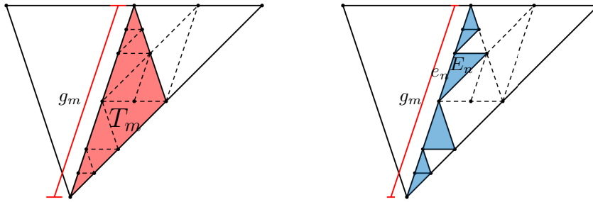
FIG 5. The edge g_m of the ancestor T_m of E (left). The partition of g_m into edges e_n of elements E_n \in \mathcal{T} (right).
