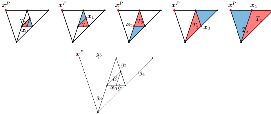
FIG 4. The chain of ancestors of E = T_0 leading to T_5 having a proper node as a vertex (above). The path g_1 \rightarrow g_2 \rightarrow \dots \rightarrow g_5 connecting x_0 \in E to the proper node x^P \in T_5 (below).
