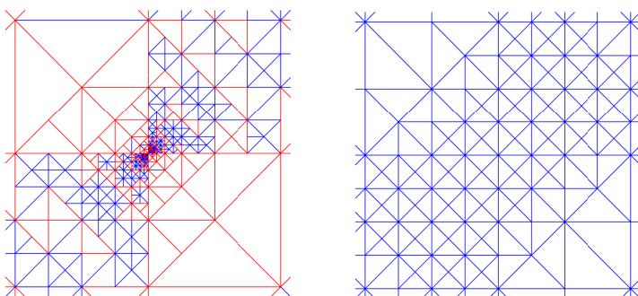
FIG 11. Test 2. Left: final grid \mathcal{T}_{\text{VEM}} . Right: final grid \mathcal{T}_{\text{FEM}} . Zoom to (-10^{-9}, 10^{-9})^2 . Mesh elements having more than three vertices are drawn in red.
