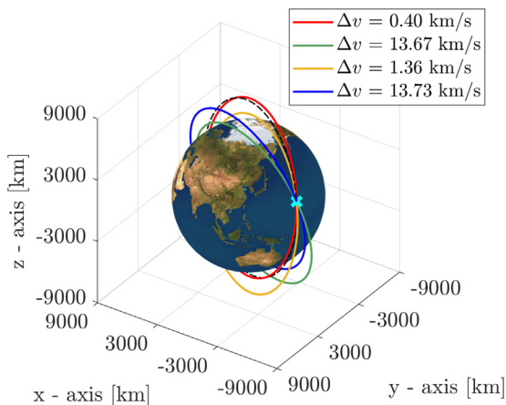
Fig. 11. Four possible intersections between parent orbit and fragments' orbit.
