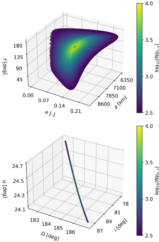
Fig. 6. Density distribution p_{v,x} as function of the Keplerian elements.
