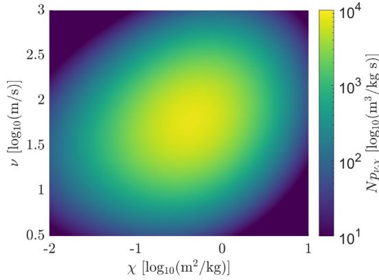
Fig. 1. Density distribution in (\chi, \nu) for a rocket body explosion.
