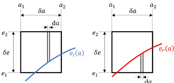
Fig. 10. Bin crossed by intersection and re-entry curves.
