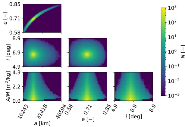
Fig. 13. Phase space density distribution in the subset of the independent variables x , at fragmentation epoch.
