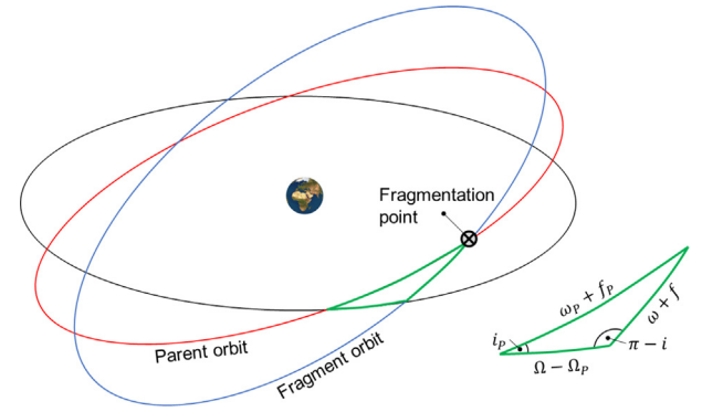
Fig. 7. Intersection between parent and fragments orbit.
