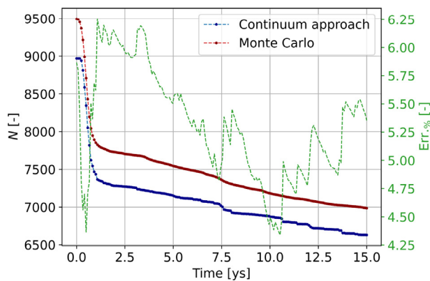
Fig. 15. Number of in-orbit fragments over time, comparison between continuum formulation and Monte Carlo simulation.
