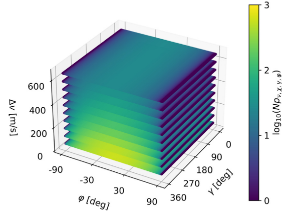
Fig. 5. Density distribution p_{v,\chi,\gamma,\phi} as function of ejection velocity magnitude \Delta v and angles \gamma , \phi .
