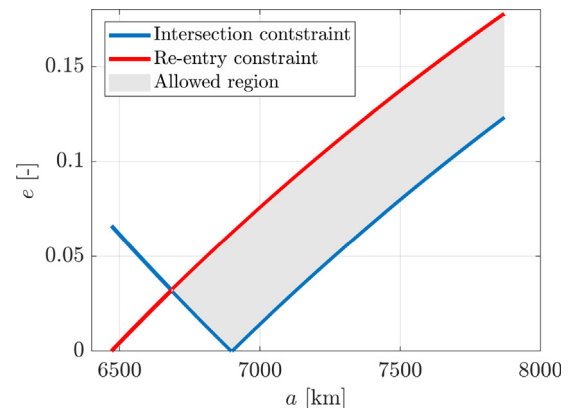
Fig. 9. Intersection and re-entry constraints for a fragmentation in LEO.
