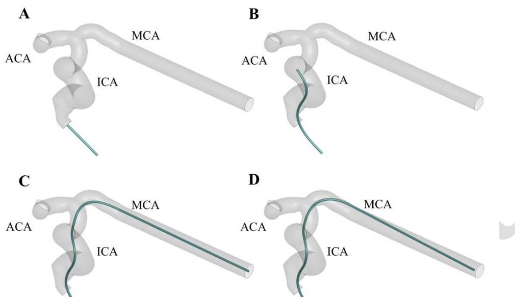
Figure 2. Steps of the tip-dragging method. A) The microcatheter is aligned with the ICA entrance. B) The tip is dragged along the vessel centerline. C) The tip of the microcatheter reaches the end position in the MCA-M1 segment. D) In the absence of external forces or constraints, the microcatheter accommodates in the vessel governed by its elastic properties until it reaches an equilibrium position. ACA, anterior cerebral artery; ICA, internal carotid artery; MCA, middle cerebral artery.
