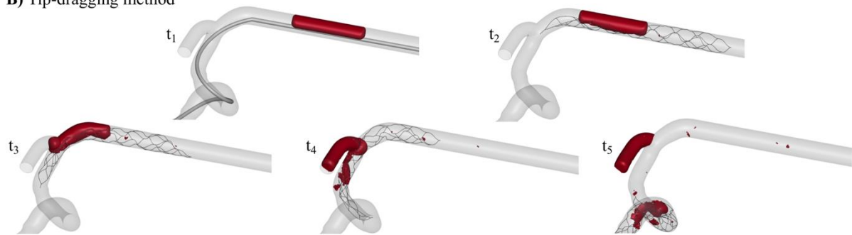
Figure 8. Thrombectomy outcomes for Patient III. Results of the thrombectomy simulations at the end of the microcatheter tracking ( t_1 ), at the end of the stent deployment ( t_2 ), and during the retrieval ( t_3 to t_5 ) for A) the centerline method and B) the tip-dragging method.
