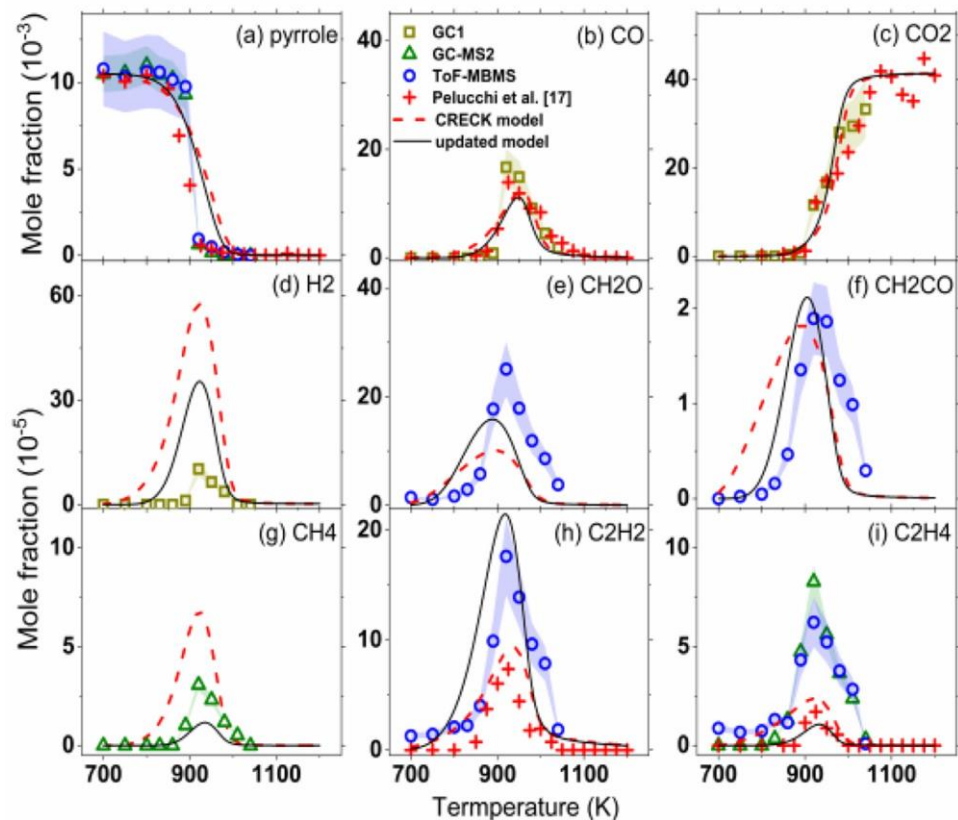
Fig. 1. Mole fraction versus temperature profiles of the reactants, main products, and small hydrocarbon intermediates. JSR conditions: fuel concentration 1.05%, \phi=0.5 , p = 1 bar, \tau=2.0 s. The red crosses represent the experimental data from Pelucchi et al. [17].
