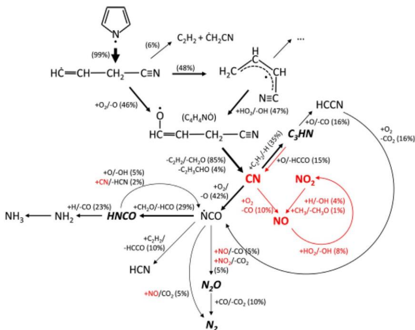
Fig. 3. Rate of production analysis of the updated model at T = 925 K, \phi = 0.5 , p = 1 bar, \tau = 2.0 s highlighting the main NO and NO 2 formation pathways. Species in bold italics are abundant species (Fig. S12, SM-1) according to model predictions that are not experimentally measured.
