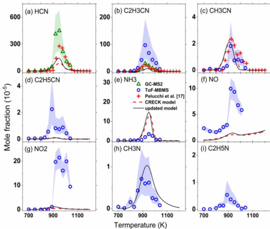
Fig. 2. Mole fraction versus temperature profiles of quantified small N-containing intermediates. JSR conditions: fuel concentration 1.05%, \phi=0.5 , p = 1 bar, \tau=2.0 s. The red cross data is taken from Pelucchi et al. [17].
