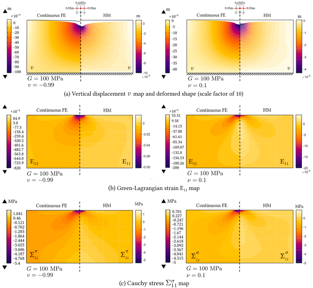
Fig. 8. Numerical results of a FE continuum vs HM model for an auxetic ( G = 100 MPa and \nu = -0.99 ) and non-auxetic ( G = 100 MPa and \nu = 0.1 ) material: (a) vertical displacement v map and deformed shape (scale factor of 10); (b) Green-Lagrangian strain E_{11} map; and (c) Cauchy stress \Sigma_{11}^{\sigma} map.
