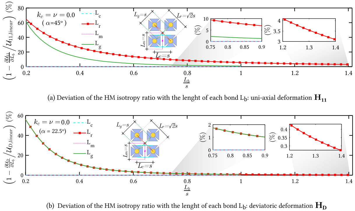
Fig. 7. Relative deviations of the HM isotropy ratio in function of the bonds length L_b , b = \{c, m, r, g\} . PS hypothesis with a \nu = 0.0 , a k_c = 0 and a deformation level of 10% were considered for: (a) \mathbf{H}_{11} deformation ( \alpha = 45^\circ ) and (b) \mathbf{H}_D deformation ( \alpha = 22.5^\circ ).
