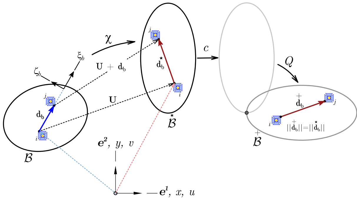
Fig. 2. Relation between reference B , elastic B^* , and transformed B^+ (Euclidean transformation) configurations.
