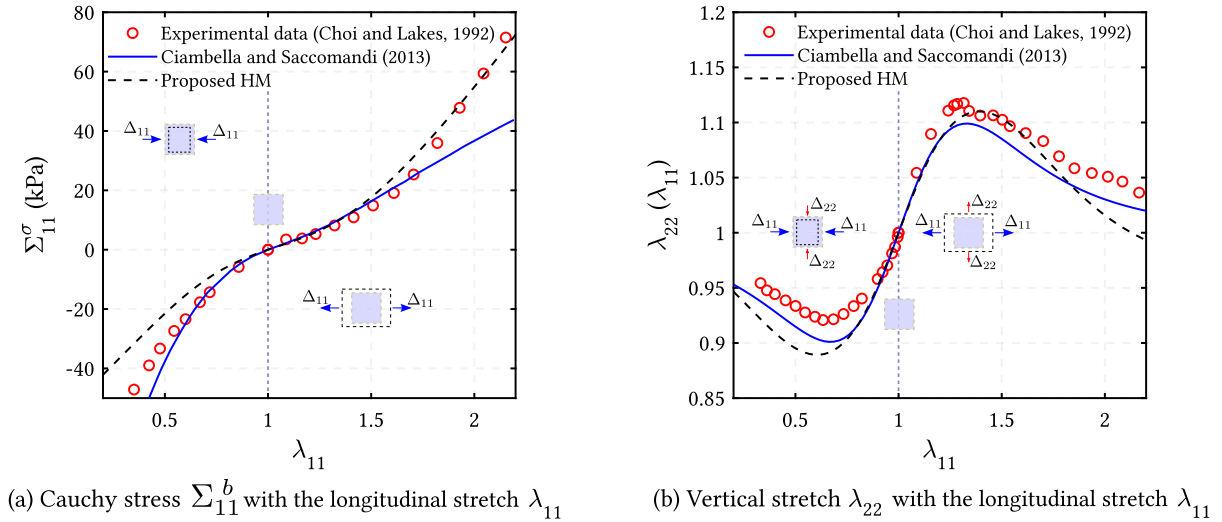
Fig. 10. Comparison between the proposed HM and the analytical [54] model with experiments data of an auxetic foam under uni-axial loading [61]: (a) Cauchy stress \sigma_{11} , and (b) evolution of the vertical (transverse) stretch \lambda_{22} with the longitudinal stretch \lambda_{11} .
