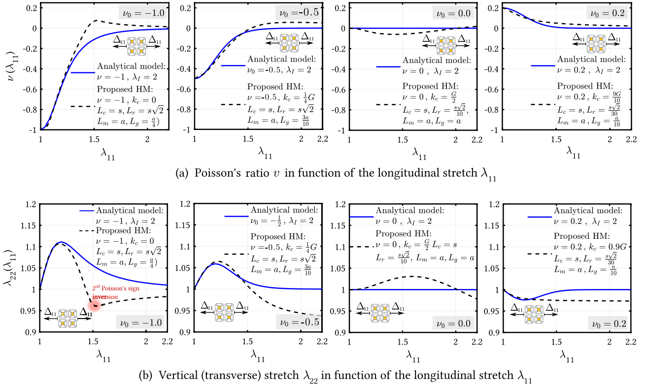
Fig. 11. Proposed HM model vs analytical model from Ciambella and Saccomandi [54]: (a) Poisson's ratio \nu in function of the uni-axial tensile stretch \lambda_{11} ; and (b) transverse stretch \lambda_{22} in function of the uni-axial stretch \lambda_{11} .
