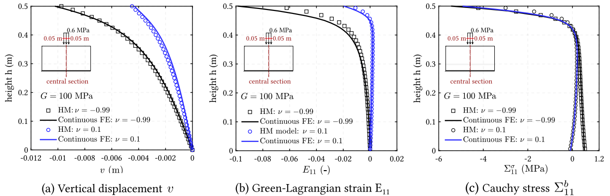
Fig. 9. Mid-section profiles of (a) vertical displacement v , (b) Green-Lagrangian strain E_{11} , and (c) Cauchy stress \Sigma_{11}^{\sigma} for both the non-auxetic and auxetic materials.
