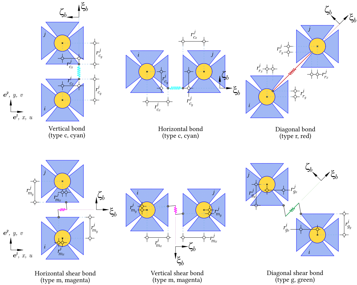
Fig. 1. Conceptual scheme of the adopted two-dimensional bonds between adjoining atoms: vertical and horizontal line bonds (cyan), diagonal line bond (red), horizontal and vertical shear bond (magenta), and diagonal shear bond (green).
