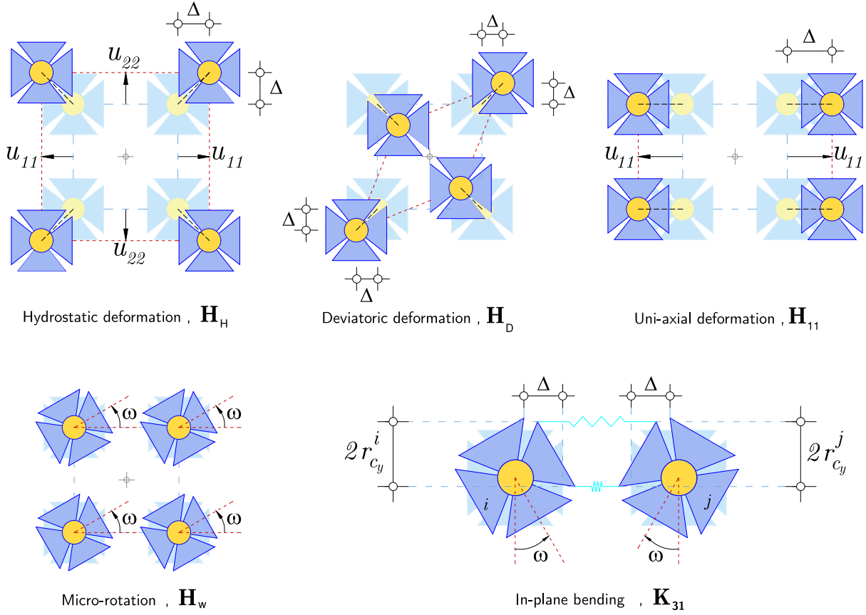
Fig. 5. Homogeneous deformation fields adopted in the energy equivalence: hydrostatic \mathbf{H}_H , deviatoric \mathbf{H}_D , uniaxial \mathbf{H}_{11} , micro-rotation \mathbf{H}_w and in-plane bending \mathbf{K}_{31} .
