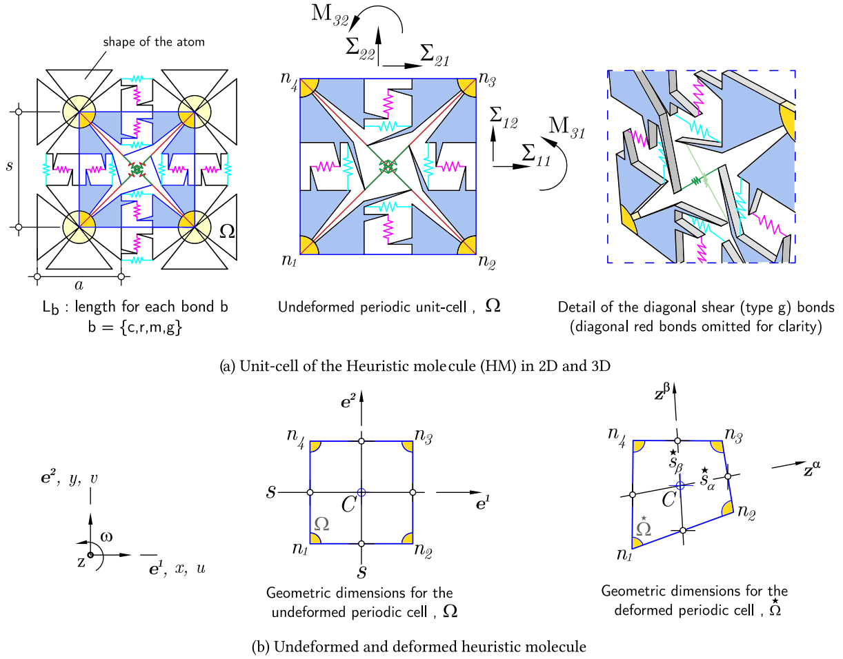
Fig. 4. Topology of the adopted heuristic molecule (HM): (a) general unit-cell in the reference configuration (2D and 3D view); and (b) general dimensions for both undeformed \Omega and deformed \Omega^* configurations.
