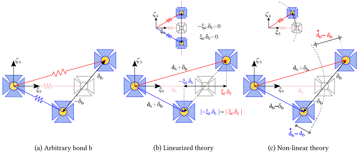
Fig. 3. Single bond b subjected to (a) a symmetric relative displacements \delta_b and -\delta_b . Description of the elastic deformation energies U_b and locus for zero-energy configurations for both (b) linearized and (c) non-linear cases.
