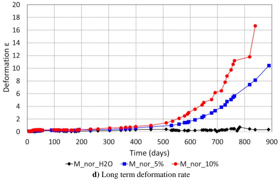
Fig. 6. M_{nor} : behavior recorded for the three aggressive agents tested
