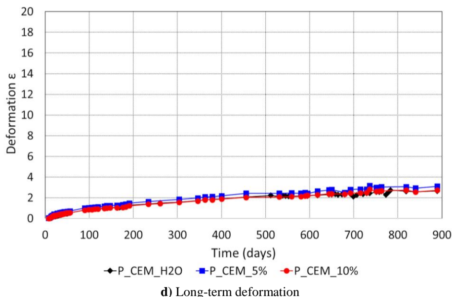
Fig. 2. P_CEM behavior for the three aggressive agents tested
