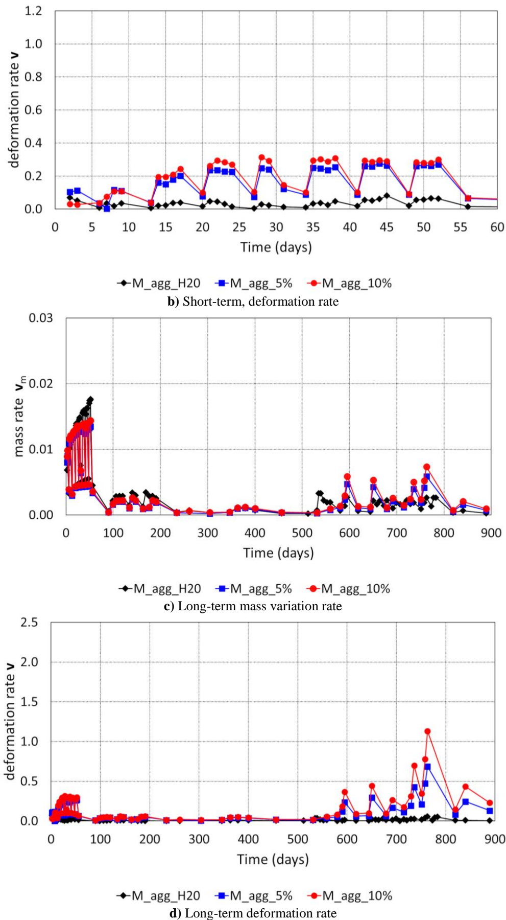
Fig. 5. M_{agg} .: rate of deformation and mass variation over time due to three aggressive agents
