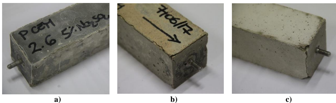
Fig. 8. Visual observations of the damage reported by the specimens immersed in a saline solution with a concentration 5% of sodium sulphate ( \text{Na}_2\text{SO}_4 ) after 600 days of testing. a) P_CEM; b) Samples M_agg; c) Samples M_nor.
