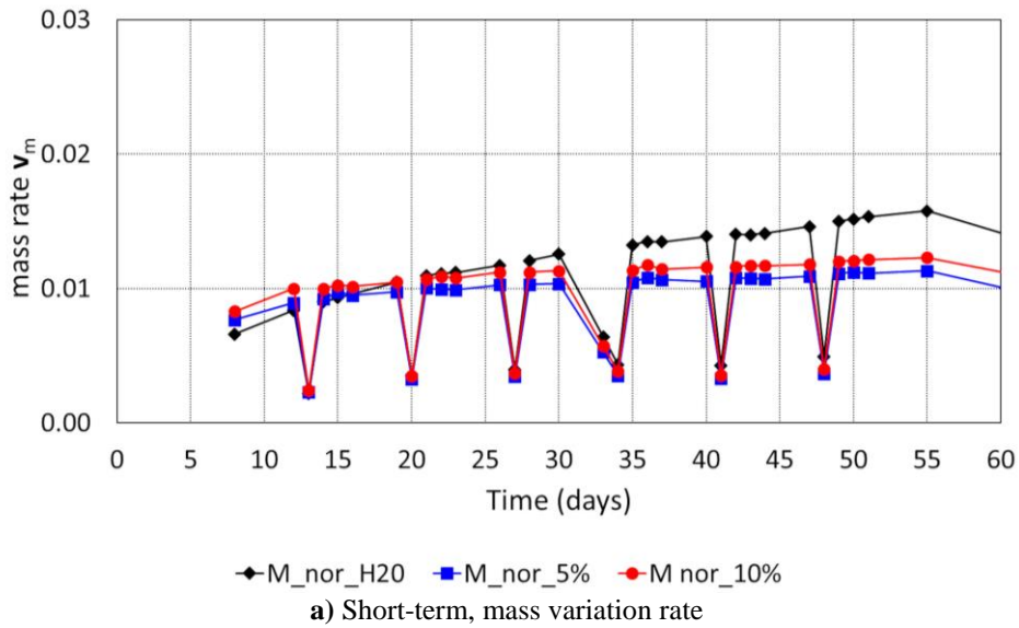
Fig. 6. M_{nor} : behavior recorded for the three aggressive agents tested
