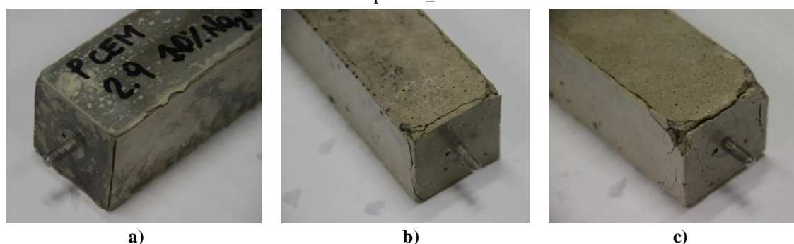
Fig. 9. Visual observations of the damage reported by the specimens immersed in a saline solution with a concentration 10% of sodium sulphate ( \text{Na}_2\text{SO}_4 ) after 600 days of testing. a) P_CEM; b) Samples M_agg; c) Samples M_nor.
