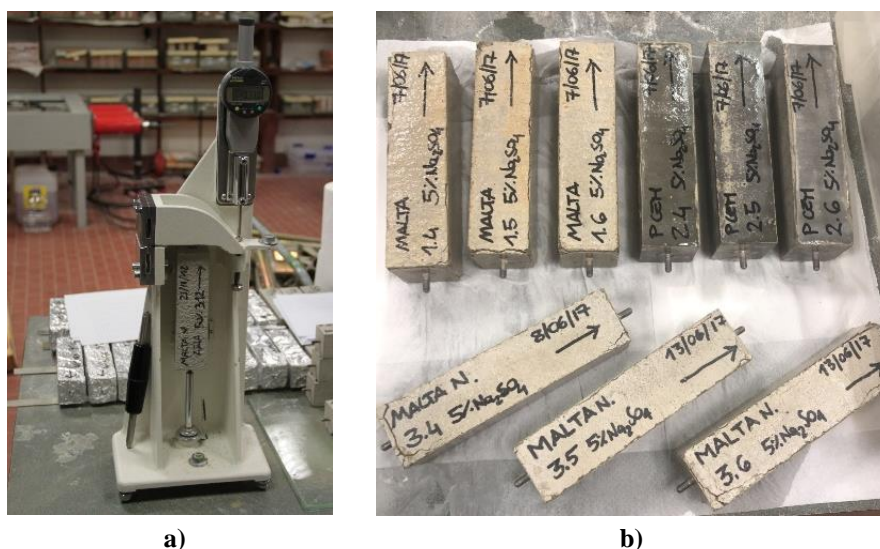
Fig. 1. a) Samples during the measurement phase; b) Samples during the last curing period
