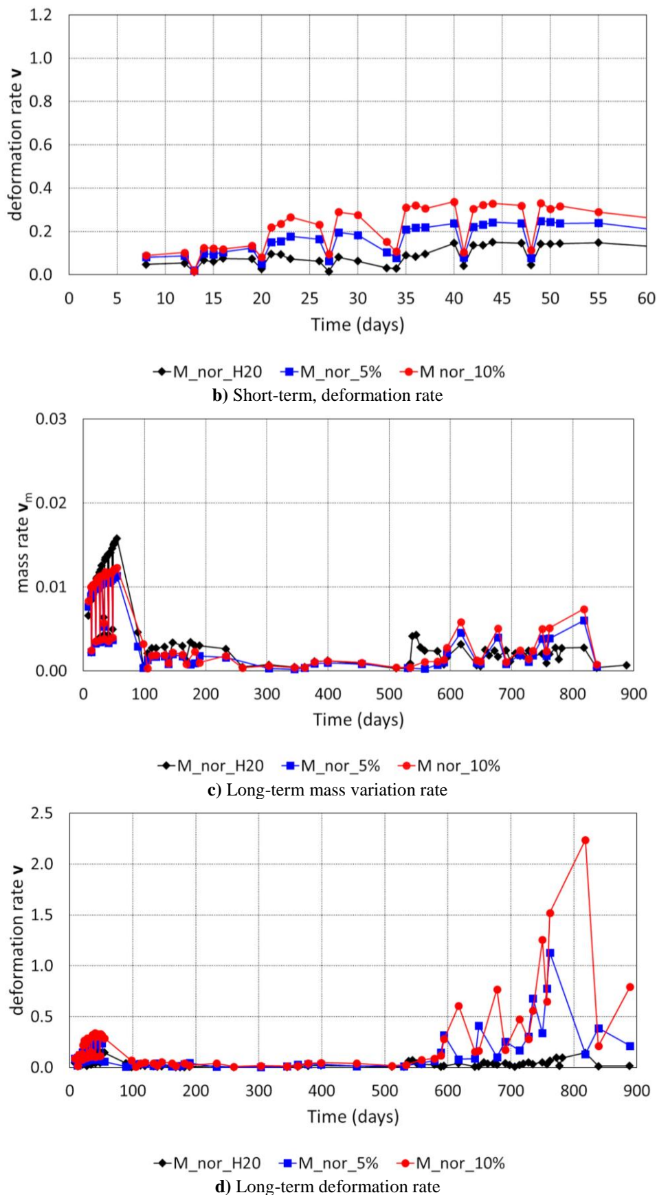
Fig. 7. M_nor.: rate of deformation and mass variation over time due to three aggressive agents The observations made in the previous paragraphs on the probable evolution of the damage starting from the results obtained in reading the evolution of the deformation rate and of the variation 000014-15
