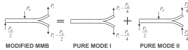
Fig. 16 Modified MMB specimen as a superposition of pure mode I and mode II loadings.
