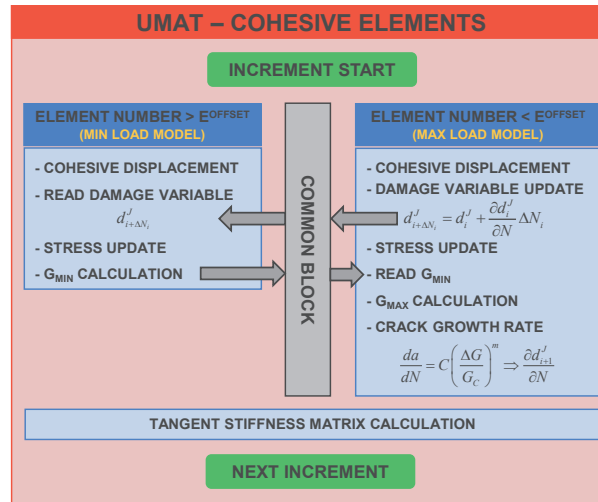
Fig. 4 Fatigue damage model implemented in ABAQUS UMAT subroutine.
