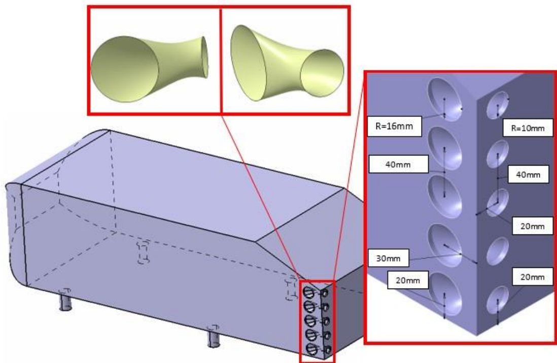
Fig 1. linking tunnels (passive flow control) on a 25° Ahmed body model [6]
