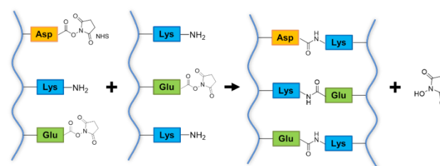
Scheme 1. Schematic outline of zero-length cross-linking between proteins, mediated by EDC/NHS activation.
