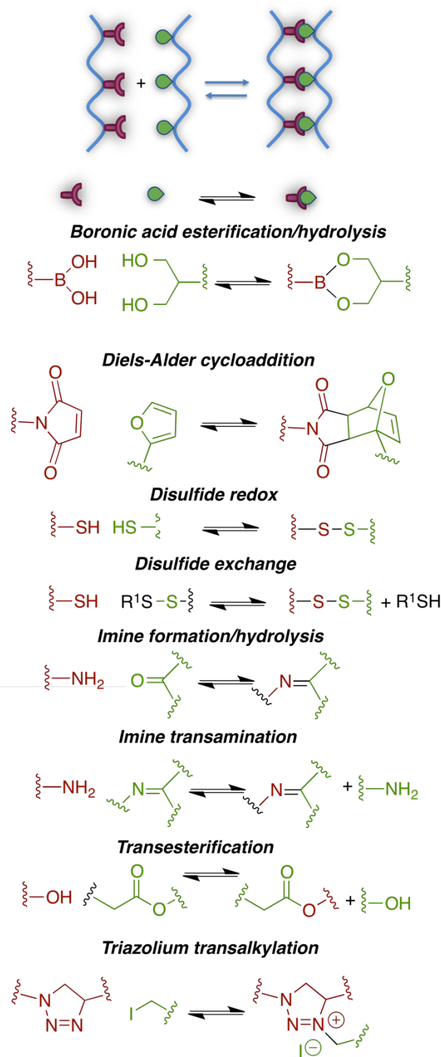
Scheme 13. Selected chemical reactions useful for dynamic cross-linking..
