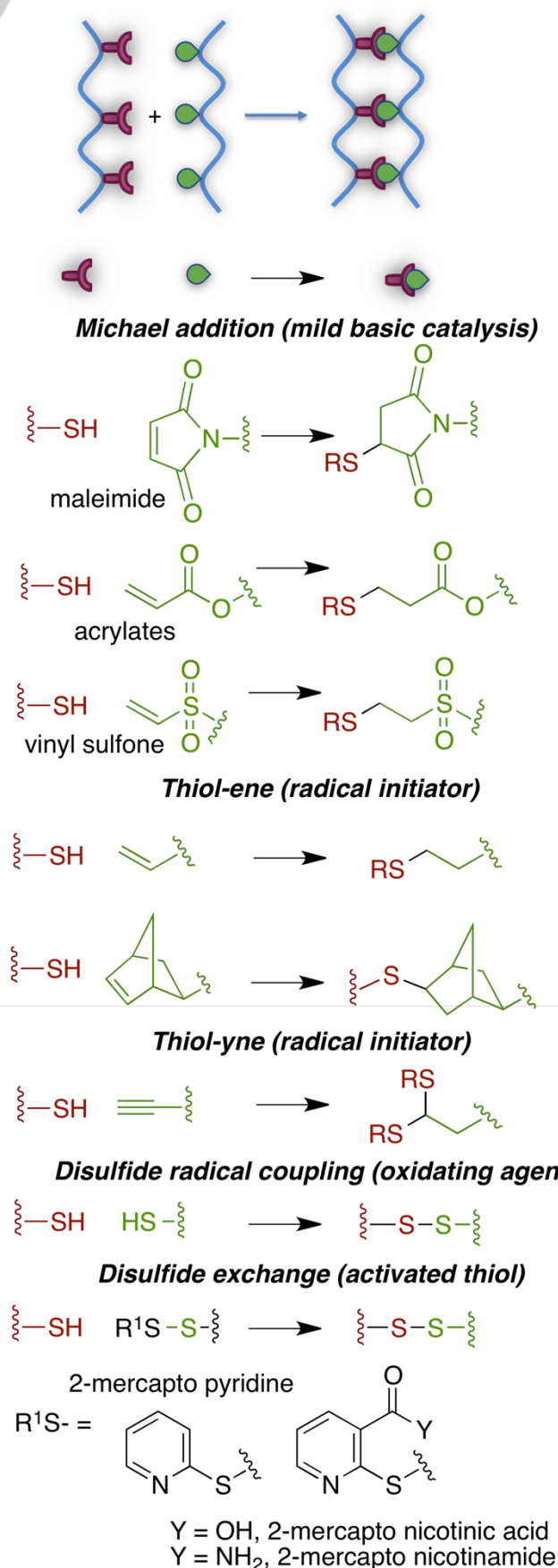
Scheme 9 Main thiol-based click reactions for hydrogel preparation.
