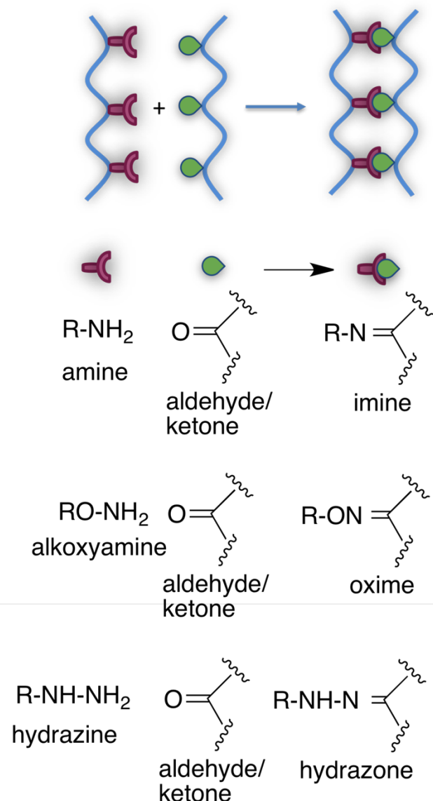
Scheme 4. Schiff base cross-links for hydrogel preparation.
