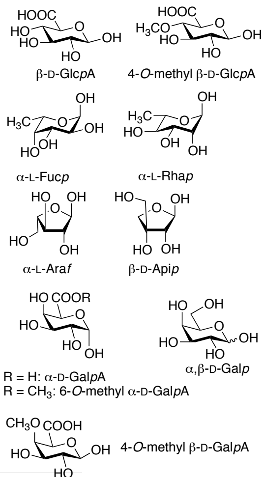
Figure 6. Main monosaccharides units composing pectins.
