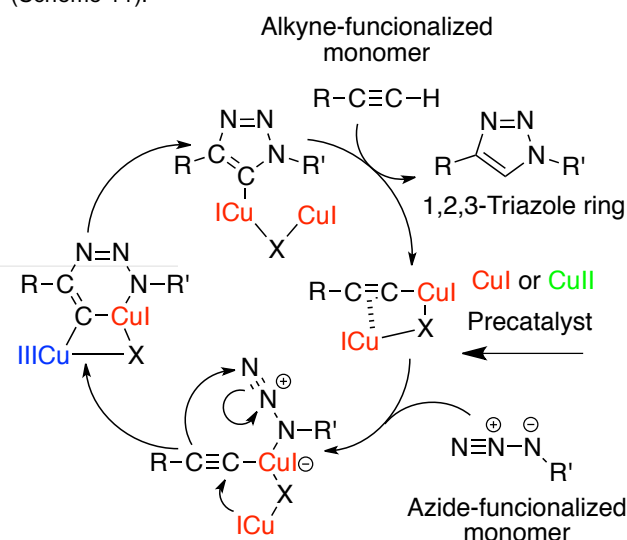
Scheme 11. Current proposed mechanism for the CuAAC reaction.
