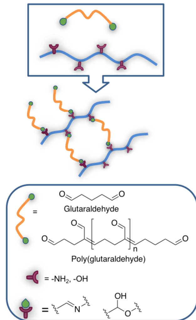
Scheme 5. Glutaraldehyde cross-linking products.
