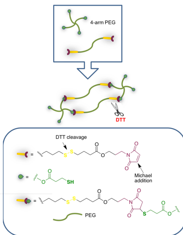
Scheme 16. Chemo-orthogonal chemistry in redox-responsive hydrogels.
