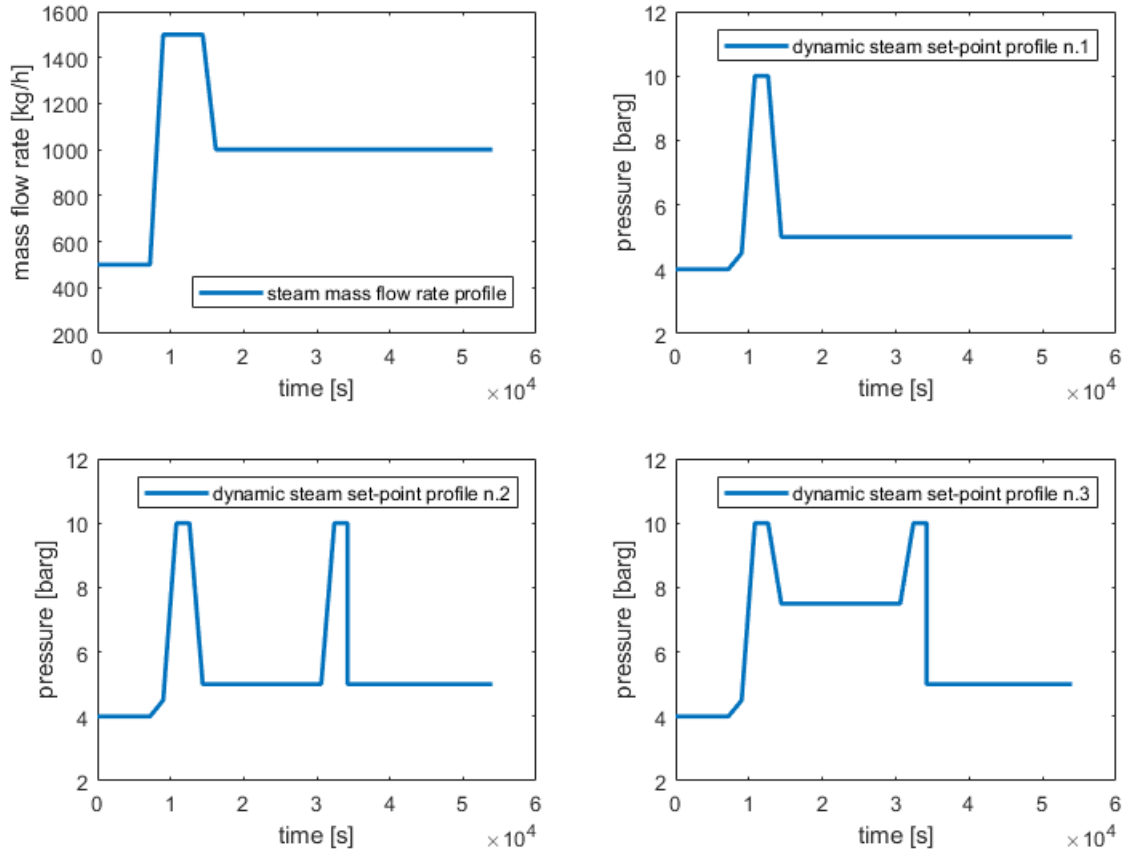
Figure 3: The daily variations in the steam mass flow rate and the desired pressure levels of the considered end-users
