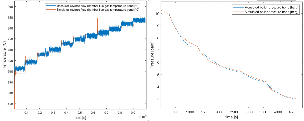
Figure 2: Comparison between the simulated values of reverse flow chamber temperature and the experimental data, while supplying different steam flow rates (left) and the comparison between the simulated transient boiler pressure profiles with the experimentally measured data, while undergoing an instantaneous steam extraction valve opening (from the results of the validation procedure performed and presented in [48])
