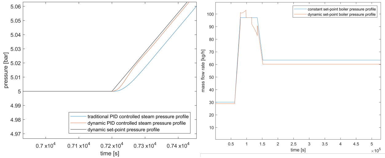
Figure 4: The comparison between the steam pressure profiles (left) and between the required hourly fuel flow rate (right), while employing the constant-setpoint and multi-setpoint strategies
