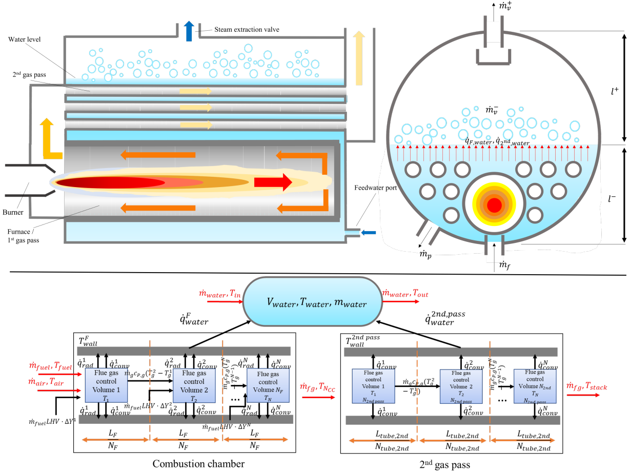
Figure 1: A simplified schematic representation of a fire-tube boiler longitudinal section (upper-left), cross-section (upper-right) equipped with a SPRF combustor and the employed finite element modelling architecture (bottom) for the flue-gas side along furnace and second gas pass longitudinal direction
