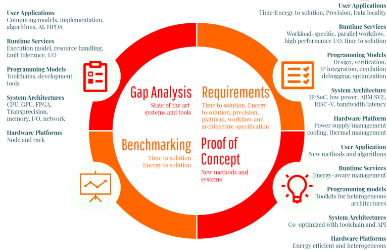
Figure 2: The TEXTAROSSA Co-Design Approach
