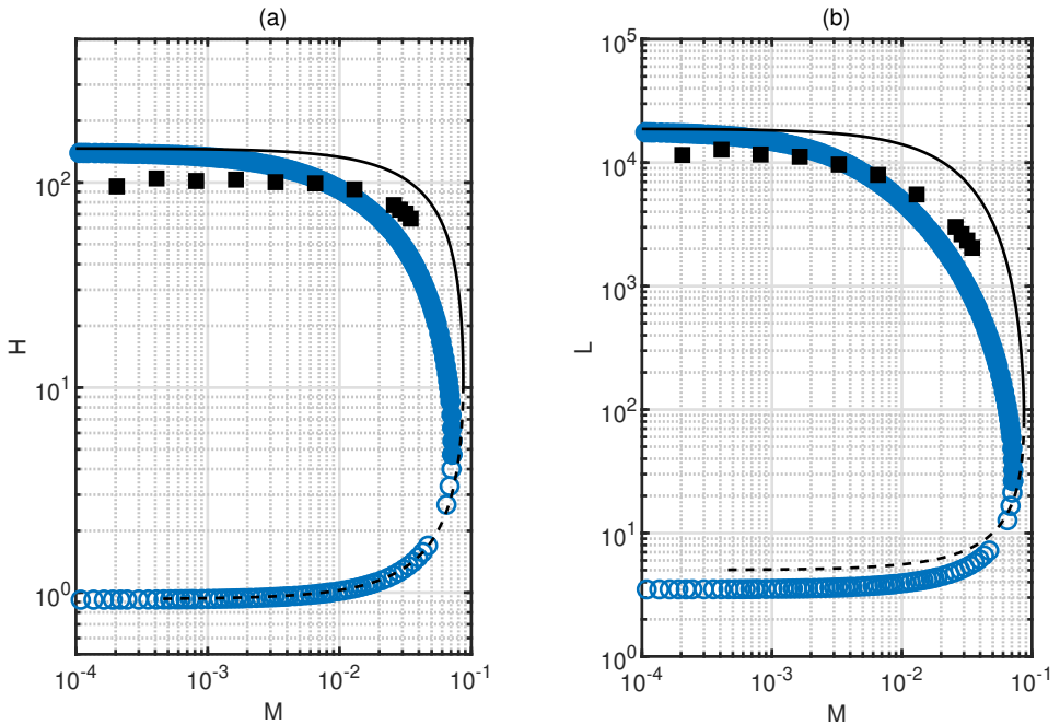
Figure 5: Average trajectory (a) height and b) length as functions of the mass hold-up, when St = 100 and Sh = 0.05 . Same legend as in figure 3.
