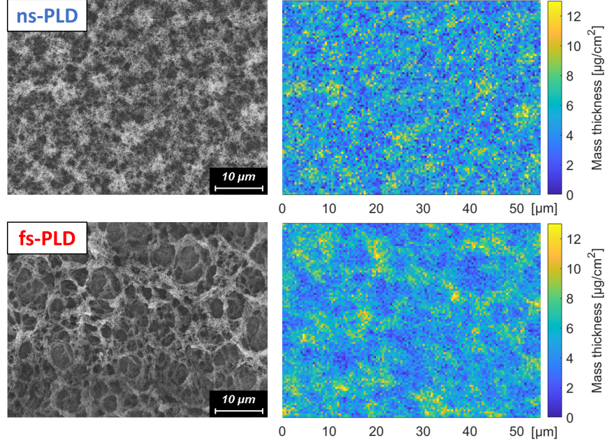
Figure 8: SEM images (on the left) and corresponding mass thickness maps (on the right) for carbon foam produced by nanosecond and femtosecond PLD, top and bottom respectively. The samples have the same average mass thickness ( \sim 5 \mu\text{g}/\text{cm}^2 ) and density ( \sim 6 \text{ mg}/\text{cm}^3 ).
