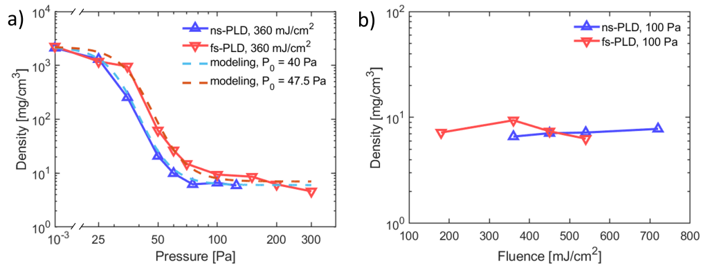
Figure 12: Mean density of carbon films deposited with ns-PLD (blue) and fs-PLD (red) with a deposition time of 10 minutes. a) Density as a function of background Ar pressure, with constant laser fluence equal to 360 mJ/cm². Dotted lines are obtained via equation 3.4. b) Density as a function of laser fluence, with constant background Ar pressure of 100 Pa.
