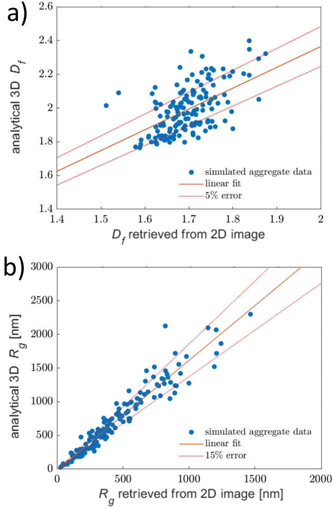
Figure 1: a) and b) show the calibration curve for the fractal dimension D_f and the gyration radius R_g respectively, as obtained by the simulated aggregates data. The blue points coordinates are given by analytical calculation of the variable on the ordinata (3D D_f and R_g ) and the value estimated from the simulated aggregate 2D image on the abscissa (with the box counting method for D_f and the equivalent radius for R_g ), as explained in the text.
