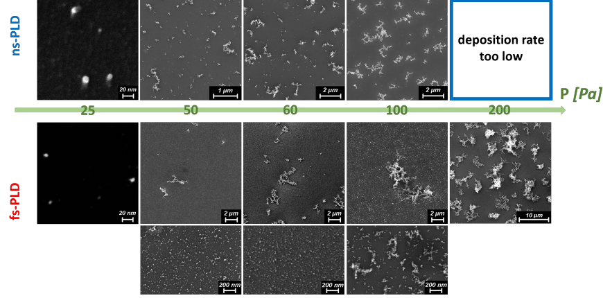
Figure 2: SEM images of the single carbon fractal aggregates, obtained with short deposition times (30 s) and displayed as a function of the background argon pressure (the fluence is fixed at 360 \text{ mJ/cm}^2 ). The upper panels refer to ns-PLD, the middle and bottom panels to fs-PLD. The middle panels show the entire fs-PLD aggregates, with lower magnification, while the bottom panels are higher magnification images of the same sample.
