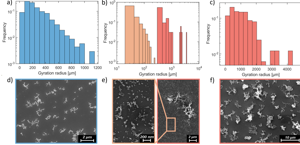
Figure 5: Typical gyration radius distributions (a-c) along with the associated SEM micrographs (d-f). Note that the ordinate values are normalized, and for panel b) the large population and the small population distributions are normalized independently. Moreover, the abscissa values are different in the three cases (and in a logarithmic scale for panel b), to better highlight the shape of each distribution. The left sample (a-d) presents a distinctive exponential distribution, typical of the ns-PLD samples, while the (b-d) panels highlight the double population in a fs-PLD sample (for both samples the deposition conditions are 360 \text{ mJ/cm}^2 and 100 \text{ Pa} ). In (c-f) another fs-PLD sample is represented, as characteristic of the peaked aggregate distributions (obtained at 360 \text{ mJ/cm}^2 and 150 \text{ Pa} ).
