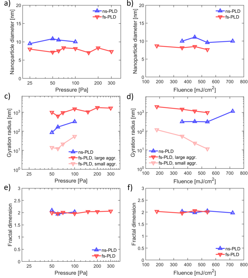
Figure 4: Results of the fractal aggregates analysis. In the left panels (a,c,e) the behaviour in respect to the argon pressure is reported, with a constant fluence of 360 mJ/cm 2 . The fluence dependence is shown in the right panels (b,d,f), with the pressure set to 100 Pa. The aggregate characteristics reported are the nanoparticle diameter d_{np} (a,b), the aggregate gyration radius R_g (c,d) and the aggregate fractal dimension D_f (e,f). For fs-PLD, the two different aggregate populations (large micrometric aggregates and small background aggregates) are considered separately. No gyration radius nor fractal dimension is reported for samples at 25 Pa, as only single nanoparticles are present in those conditions.
