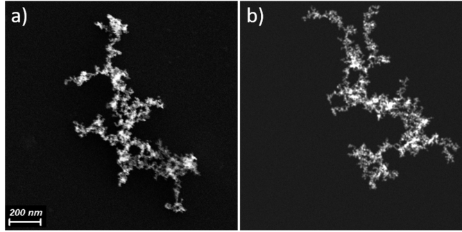
Figure A.14: Comparison between a real and a simulated fractal aggregate, the visual similarity is significant. a) is a scanning electron microscope image of a real aggregate, while b) is a simulated image of one of the aggregates constructed through the cluster-cluster aggregation (CCA) algorithm.
