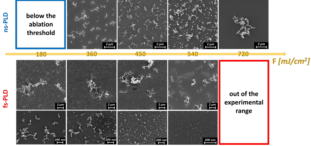
Figure 3: SEM images of the single carbon fractal aggregates, obtained with lower deposition times (30 s) and displayed as a function of the laser fluence (the argon pressure is fixed at 100 Pa). The upper panels refer to ns-PLD, the middle and bottom panels to fs-PLD. The middle panels show the entire aggregates, with lower magnification, while the bottom panels are higher magnification images of the same sample.
