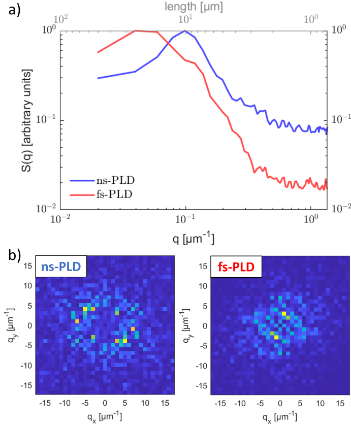
Figure 9: Structure factor S(q) retrieved from the Fourier transform of the mass thickness maps of figure 8. a) Normalized power spectrum of the ns-PLD foam (blue) and fs-PLD foam (red). b) central region of the 2D Fourier transform in the two cases.
