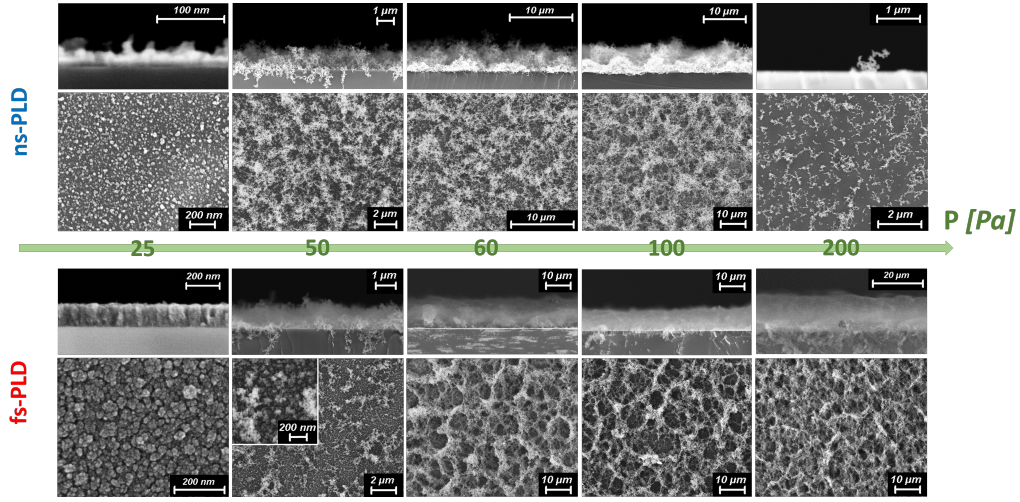
Figure 6: SEM images of carbon nanostructured films, showing the evolution of their morphology as a function of the background argon pressure in both nanosecond (upper panels) and femtosecond (lower panels) deposition regimes (to be compared with the respective aggregates of figure 2). The fluence is set to 360 \text{ mJ/cm}^2 , and the deposition time is 10 minutes. For each sample, a cross section image (top) and a plane view (bottom) are shown. For the fs-PLD sample at 50 Pa a higher magnification inset is added to highlight the peculiar mixed nature of the film.
