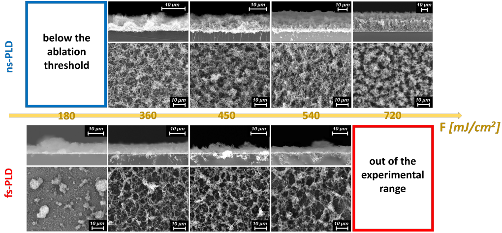
Figure 7: SEM images of carbon nanofoams, showing the evolution of their morphology as a function of the laser fluence in both nanosecond (upper panels) and femtosecond (lower panels) deposition regimes (to be compared with the respective aggregates of figure 3). The pressure is set to 100 Pa, and the deposition time is 10 minutes. For each sample, a cross section image (top) and a plane view (bottom, all at the same magnification) are shown. The range of employed fluence is limited by the ablation threshold in ns-PLD and the experimental configuration for fs-PLD.
