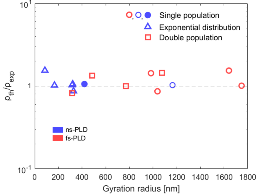
Figure 13: Ratio between the theoretical carbon foam density (calculated with the fractal scaling law starting from the aggregate properties) and the experimental average density of the respective sample, represented as a function of the gyration radius. Circles represent samples with a peaked single R_g distribution (right panel of fig. 5), triangles refer to exponential R_g distributions, and squares correspond to the double population samples. The filled round data point refer to a carbon foam we produced in different experimental conditions (pressure = 700 Pa Ar, fluence = 1.2 J/cm 2 ) in a previous work (34). A red color indicates a fs-PLD sample, while the ns-PLD ones are represented in blue.
