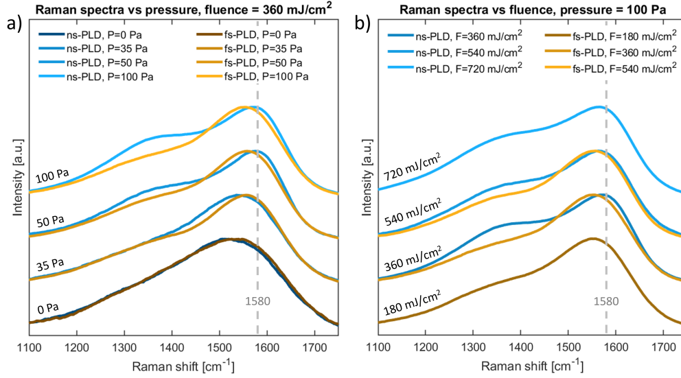
Figure 10: Normalized Raman spectra of samples deposited with ns-PLD (blue-cyan lines) and fs-PLD (red-orange lines). The vertical gray line indicates the position of the graphite G peak at \simeq 1580 \text{ cm}^{-1} . a) Fluence is fixed to 360 \text{ mJ/cm}^2 , pressure varies from high vacuum to 100 Pa. b) Pressure is fixed at 100 Pa, fluence varies from 180 \text{ mJ/cm}^2 to 720 \text{ mJ/cm}^2 .
