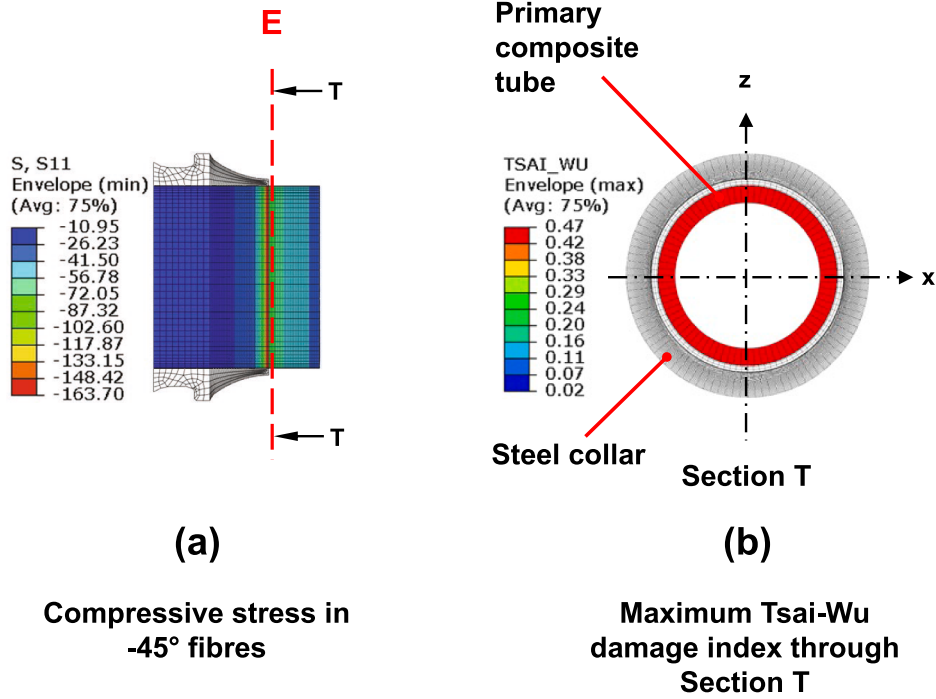
Fig. 10. Stress and damage field in the primary composite tube at Position E, due to the torsional moment, M_y (Note: secondary composite tube omitted for clarity). (a) Compressive S_{11} (fibre) stress, -45^\circ fibres. (b) Maximum Tsai-Wu damage index through the cross-sectional xz -plane (Section T).
