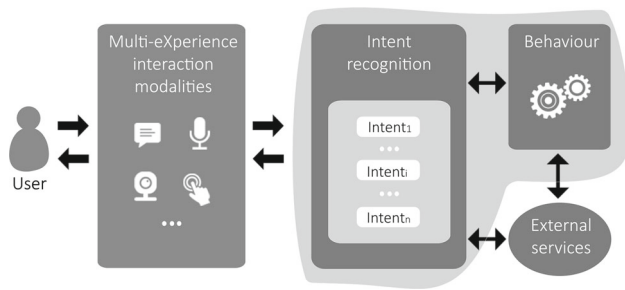
Fig. 1 Bot working schema
