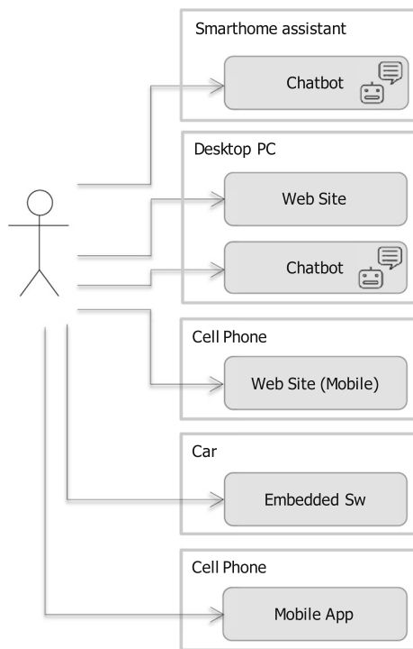
Fig. 6 Use case diagram representing a typical scenario of multiexperience user interaction
