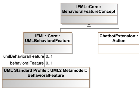
Fig. 8 IFML metamodel extension for the Chatbot Action, i.e., the corresponding IFML concept of the Action metaclass defined in the Chatbot metamodel, allowing invocation of actions in the chatbot from any UI components
