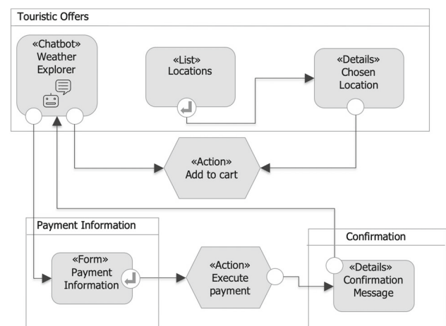
Fig. 9 IFML model example with chatbot integrated in the user navigation of a tourism web site
