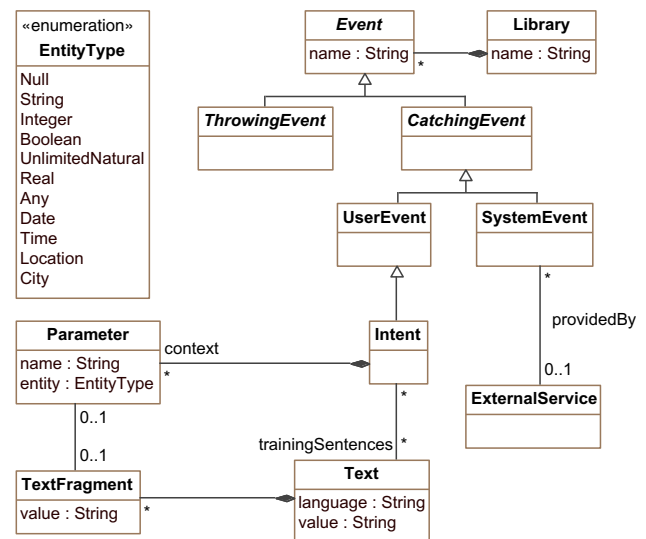
Fig. 3 Intent package metamodel
