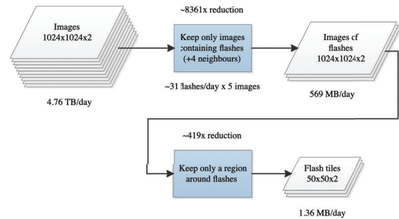
Figure 11. LUMIO payload data reduction strategy.
