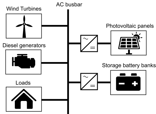
Figure 1: Microgrid architecture [17].
