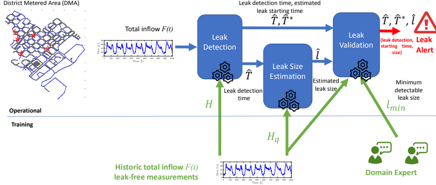
Fig. 4: Leak detection scheme, where historical leak-free flow measurements at the inlets are used as reference for leak detection and leak size estimation, and the information of those modules is used in combination with domain experts knowledge setting the minimum leak size l_{\min} to validate the leak. This picture is better interpreted in the coloured version of the paper.
