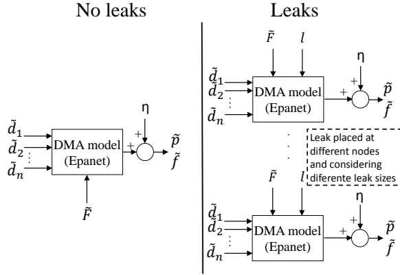
Fig. 7: Scheme of the procedure used for data generation using a hydraulic simulator. Different sequences are generated for training our classifiers where the first part is leak free while the second part introduces a leak at different nodes and for each considered leak size.
