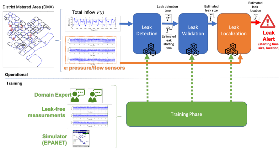
Fig. 3: An overview of the proposed solution comprising leak detection, leak validation and leak localization. All these modules are trained from a flow time series and take advantage of knowledge from domain experts. This picture is better interpreted in the coloured version of the paper.
