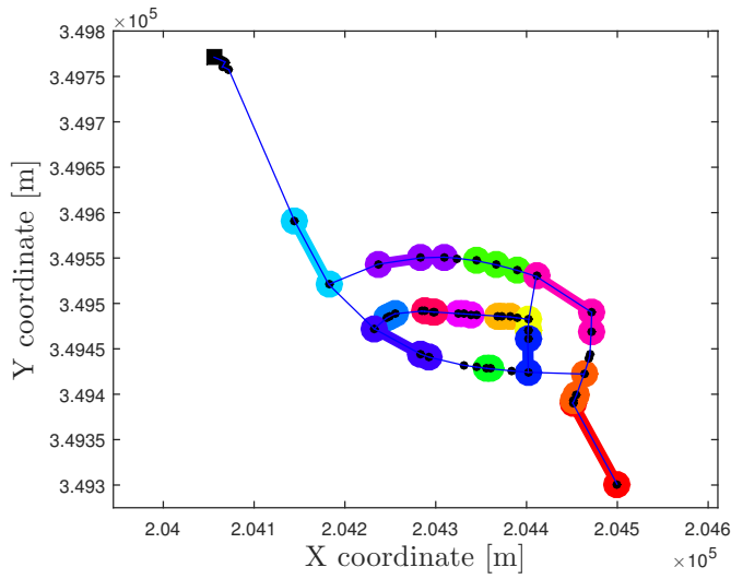
Fig. 9: Clusters formed using classifiers C^l trained on pressure sensors and medium leak. Each colour represents a different cluster. Singleton nodes of the clusters are black. This picture is better interpreted in the coloured version of the paper.
