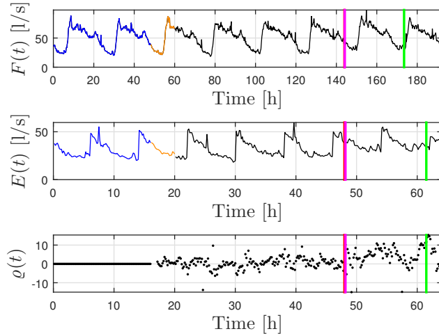
Fig. 12: Leak detection for Nova Icària DMA. This picture is better interpreted in the coloured version of the paper.
