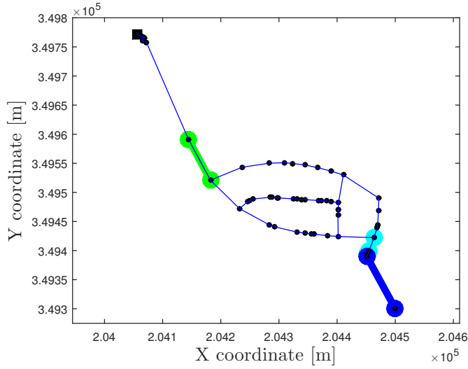
Fig. 10: Clusters formed using classifiers C^l trained on flow sensors and medium leak. Each colour represents a different cluster. Singleton nodes of the clusters are black. This picture is better interpreted in the coloured version of the paper.
