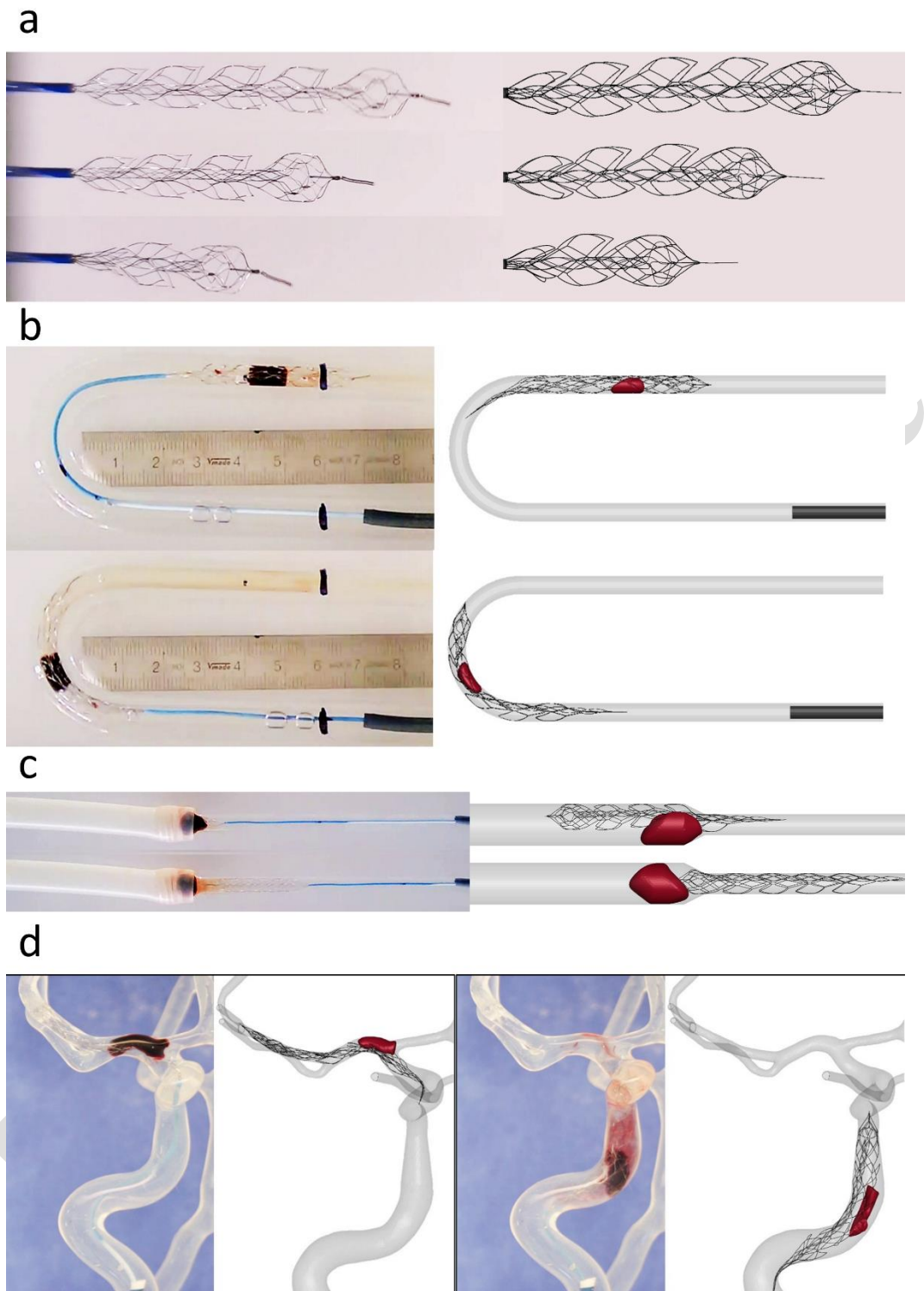
Figure 2. Validation Models: (a) crimp and release test of the EmboTrapII stent, (b) thrombectomy test in a glass U-bent vessel, (c) thrombectomy test in a silicone funnel-shaped vessel, (d) thrombectomy test in a silicone 3D-printed patient-like branch.
