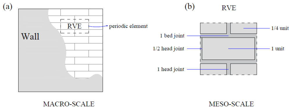
Figure 2: Schematic representation of the periodic volume element: (a) at the macro-scale or the structural level; and (b) at the meso-scale, where the homogenization procedures are performed.
