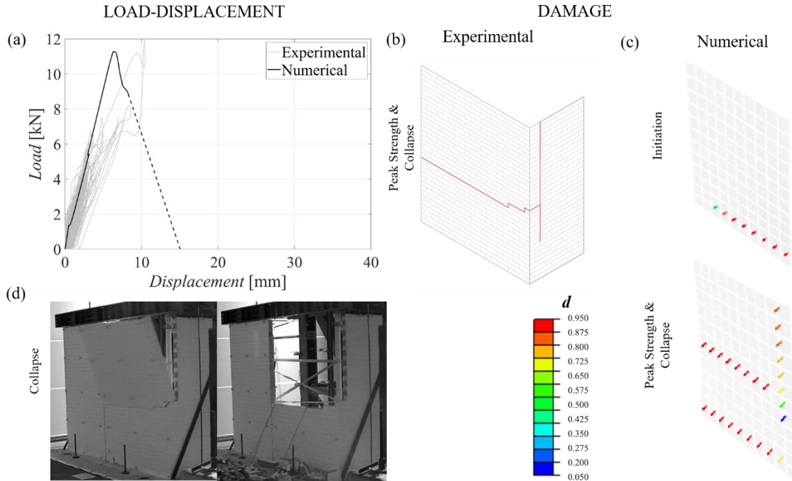
Figure 13: Comparison between the experimental and numerical response for the WU-SJ wall restrained on all two adjacent sides only (i.e. CS-000-L2 [26] in Table 1): (a) experimental and the numerical load-displacement behaviour; (b) experimental progression of damage; (c) numerical progression of damage; and (d) snapshots of the experimental collapse of CS-000-L2.
