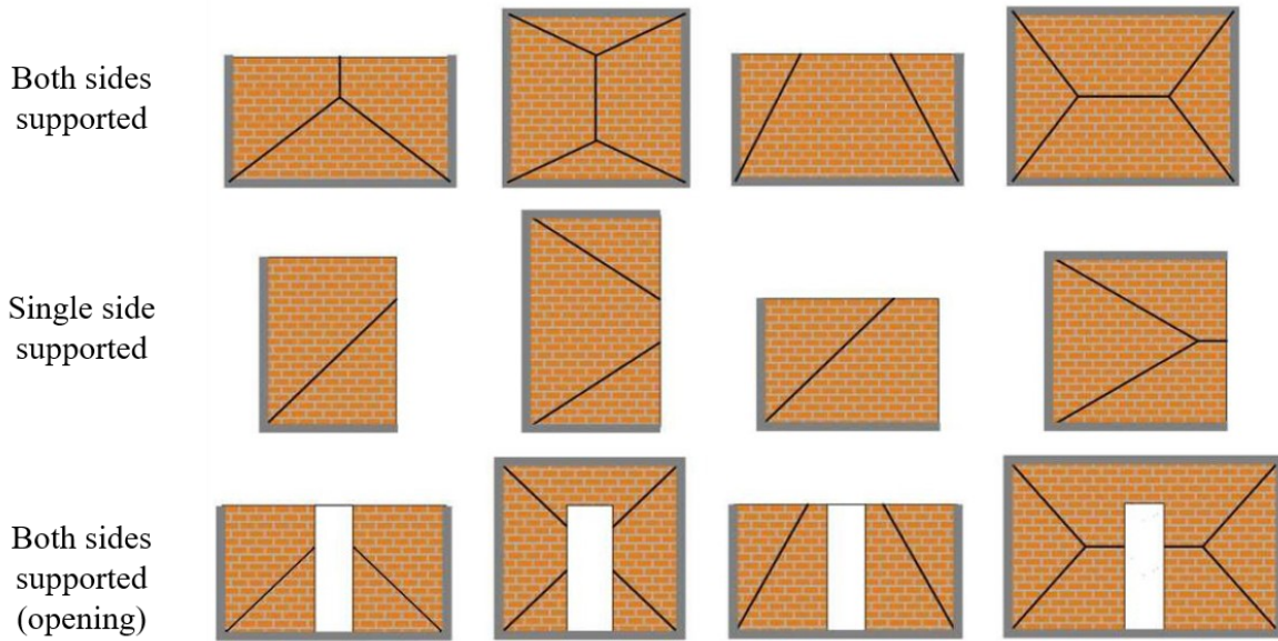
Figure 17: Failure mechanisms under out-of-plane two-way bending corresponding to various wall configurations assumed by the codified form of the virtual work method (reproduced from [104]).
