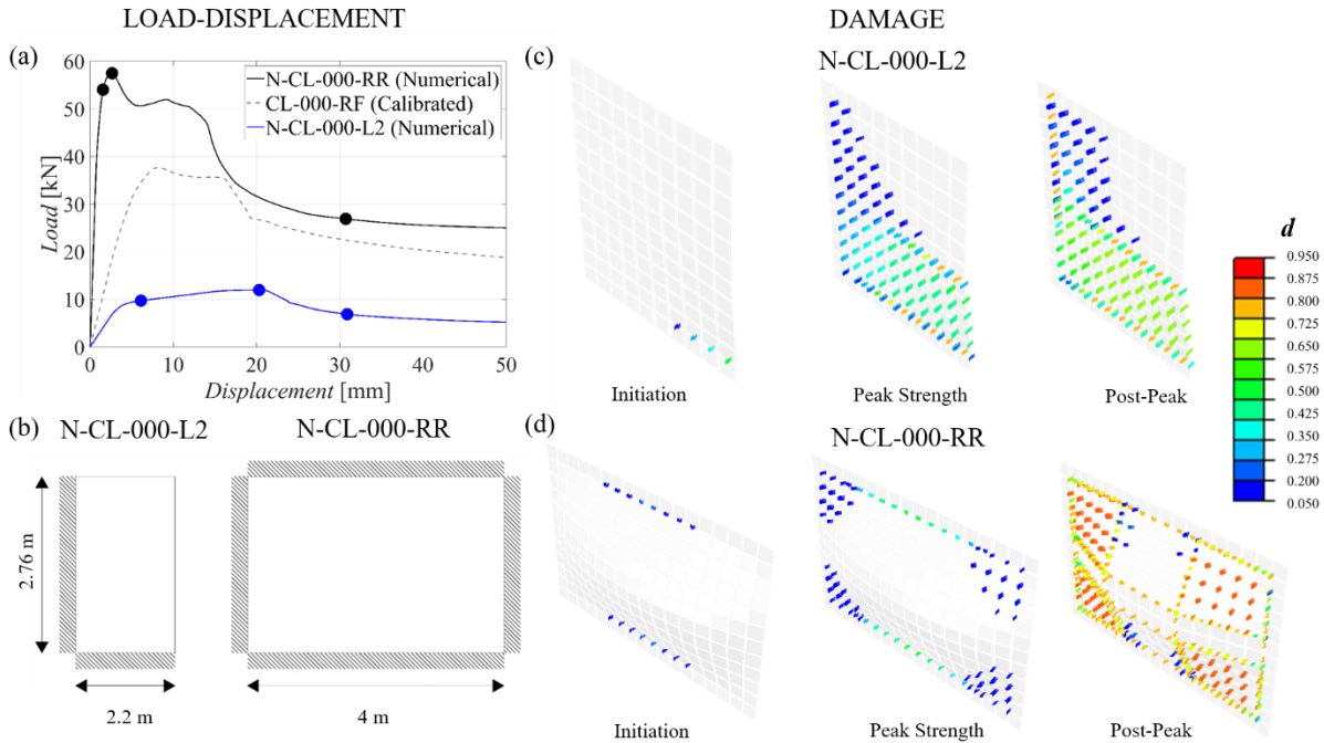
Figure 16: Numerical predictions for the SU-WJ walls hitherto untested using material properties of calibrated SU-WJ specimen (i.e. CL-000-RF [25] in Table 1): (a) numerical load-displacement behaviour; (b) dimensions and boundary conditions of the walls considered numerically; (c) numerical progression of damage for N-CL-000-L2; and (d) numerical progression of damage for N-CL-000-RR.
