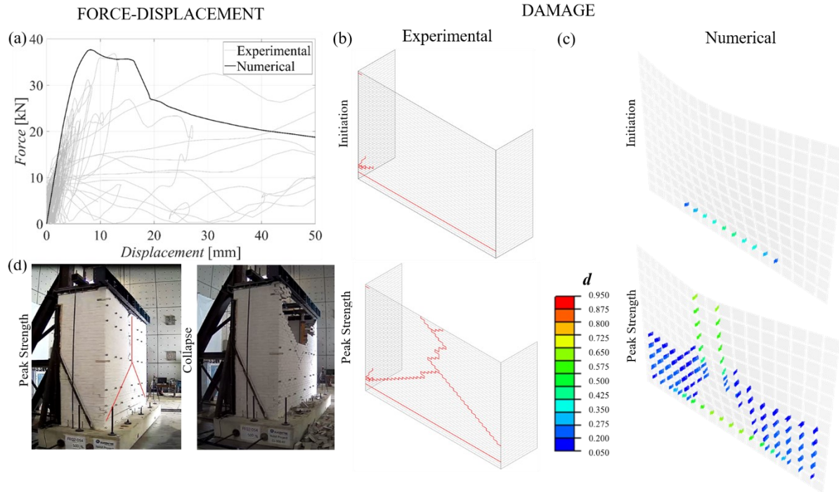
Figure 15: Comparison between experimental and numerical response for SU-WJ walls restrained on all three sides and free at the top (i.e. CL-000-RF [25] in Table 1): (a) experimental and the numerical load-displacement behaviour; (b) experimental progression of damage; (c) numerical progression of damage; and (d) snapshots of the experimental collapse of CL-000-RF.
