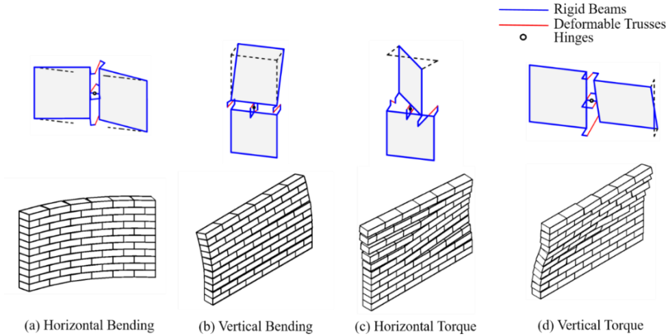
Figure 6: Deformation modes considered for the walls: (a) horizontal bending; (b) vertical bending; (c) horizontal torque; and (d) vertical torque.
