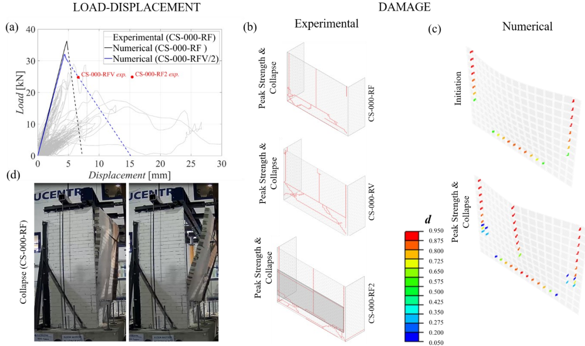
Figure 11: Comparison between experimental and numerical response for WU-SJ walls restrained on all three sides and free at the top (i.e. CS-000-RF [25], CS-000-RFV [26] and CS-000-RF2 [26] in Table 1): (a) experimental and the numerical load-displacement behaviour; (b) experimental progression of damage; (c) numerical progression of damage; and (d) snapshots of the experimental collapse of CS-000-RF.
