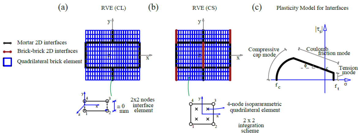
Figure 3: Detailed description of the considered RVE FE models: (a) for the SU-WJ (clay) masonry case; (b) for the WU-SJ (CS) masonry case; and (c) plasticity model used for the interfaces.
