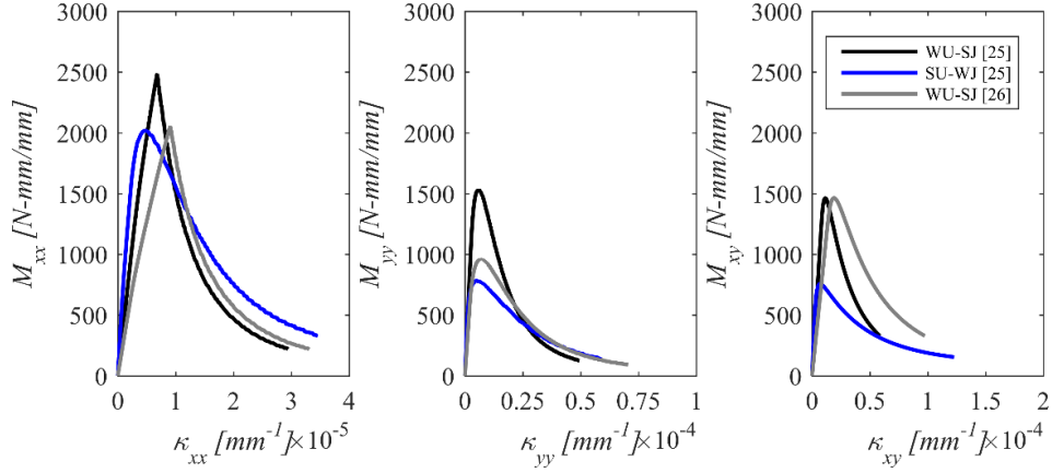
Figure 10: Moment curvature ( M - \kappa ) curves associated with all three batches of URM analysed.
