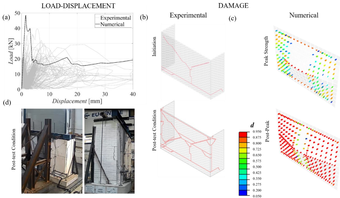
Figure 14: Comparison between the experimental and numerical response for the WU-SJ walls restrained on all four sides (i.e. CS-005-RR [25] in Table 1): (a) experimental and the numerical load-displacement behaviour; (b) experimental progression of damage; (c) numerical progression of damage; and (d) CS-005-RR at the end of testing
