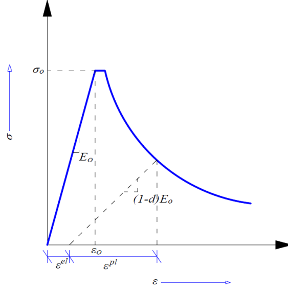
Figure 7: Parameters associated with the Concrete Damage Plasticity model.
