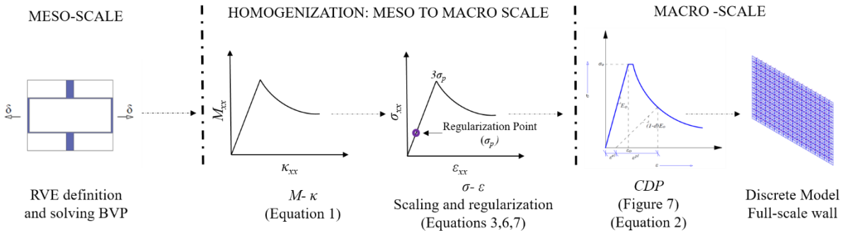
Figure 8: Scheme outlining the transferring of the material information between scales (the represented curves are hypothetical).
