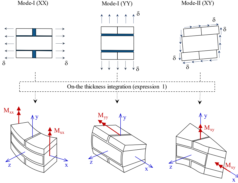
Figure 4: Deformation modes considered together with the associated output in terms of M-\kappa curves: mode-I (XX), tension along XX; mode-I (YY), tension along YY; and mode-II (XY), shear along XY.
