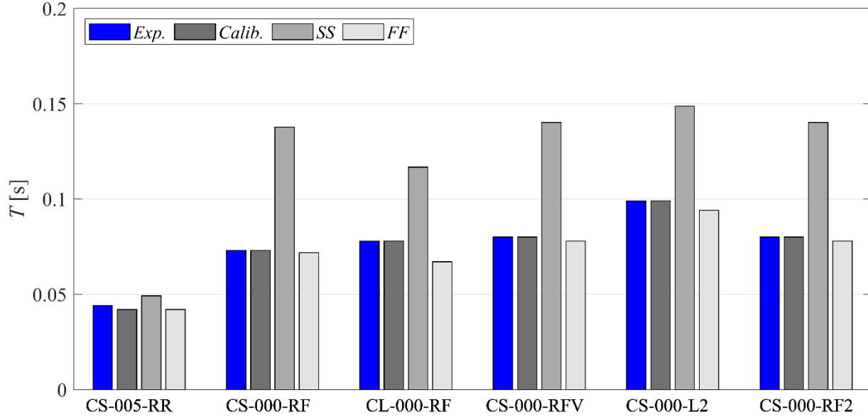
Figure 9: Comparison of the period of the first natural mode of vibration of the numerical models of the walls: calibrated ( Calib. ) vs. limiting scenarios of restraint at the vertical edges ( FF : fully fixed and SS : simply-supported) along with experimentally measured values ( Exp. )
