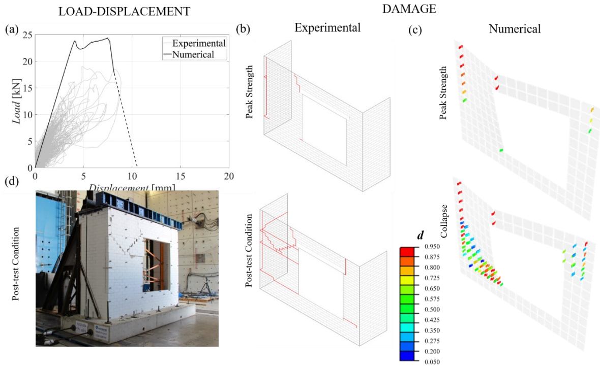
Figure 12: Comparison between the experimental and numerical response for the WU-SJ walls restrained on all three sides and free at top and with an eccentric opening (i.e. CSW-000-RF [25] in Table 1): (a) experimental and the numerical load-displacement behaviour; (b) experimental progression of damage; (c) numerical progression of damage; and (d) CSW-000-RF at the end of testing.
