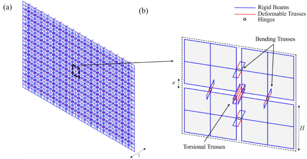
Figure 5: Assumed discrete model at a macro-scale: (a) representation of a masonry wall; and (b) its macroscopic repeating unit.
