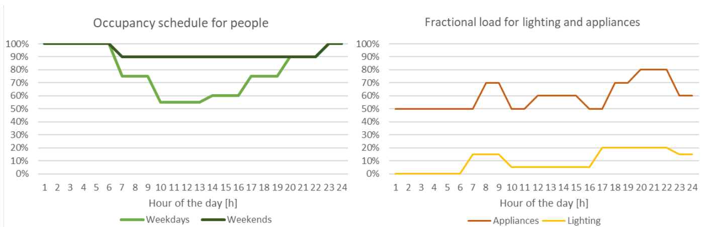
Figure 13: Fractional load schedule for occupants, lighting, and appliances for residential use
