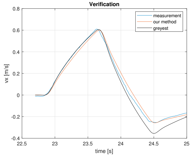
Fig. 8. Velocity model identification: verification and comparison between different methods.
