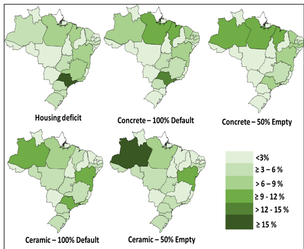
Figure 13. Percentage of the cumulative housing deficit in 2050 and CO 2 -eq emissions for each state considering each block type for the different transportation options; 100% Default—represents that the truck is loaded with 100% of its capacity and returns full; 50% empty—represents that the truck is loaded with 50% of its capacity and returns empty.
