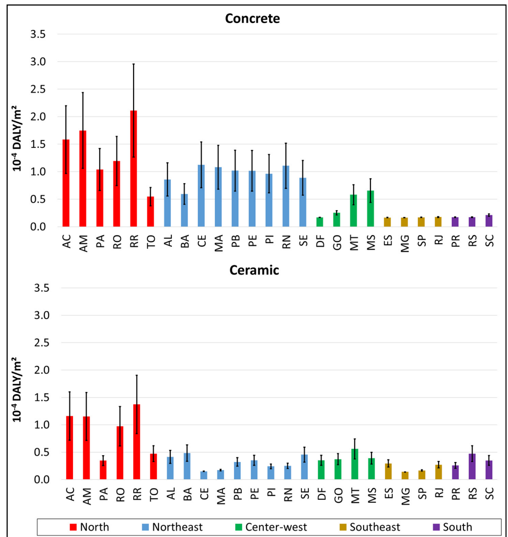
Figure 4. Total Human Health impact. The error bars represent the standard deviation due to transportation scenarios.
