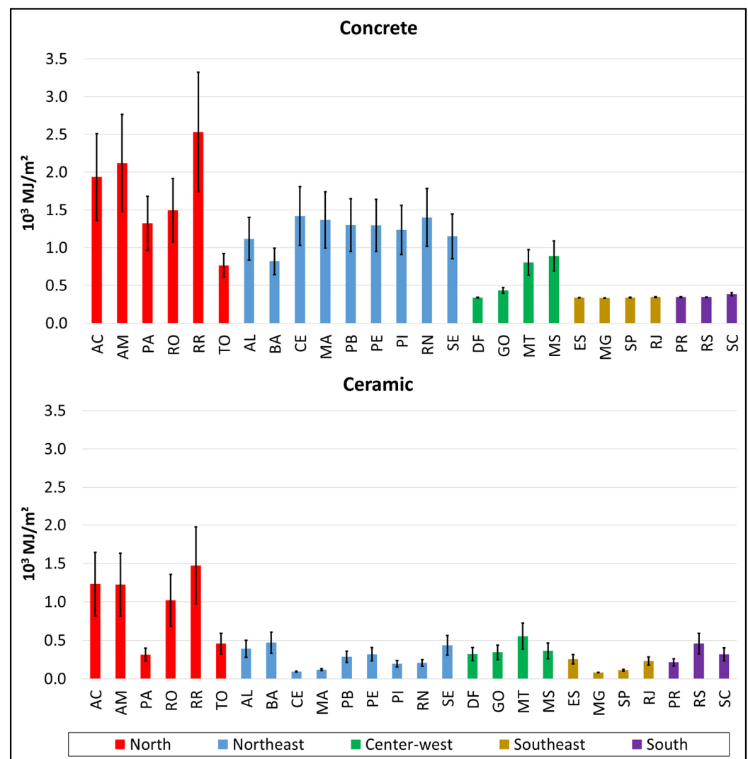
Figure 6. Total Resource Depletion impact. The error bars represent the standard deviation due to transportation scenarios.
