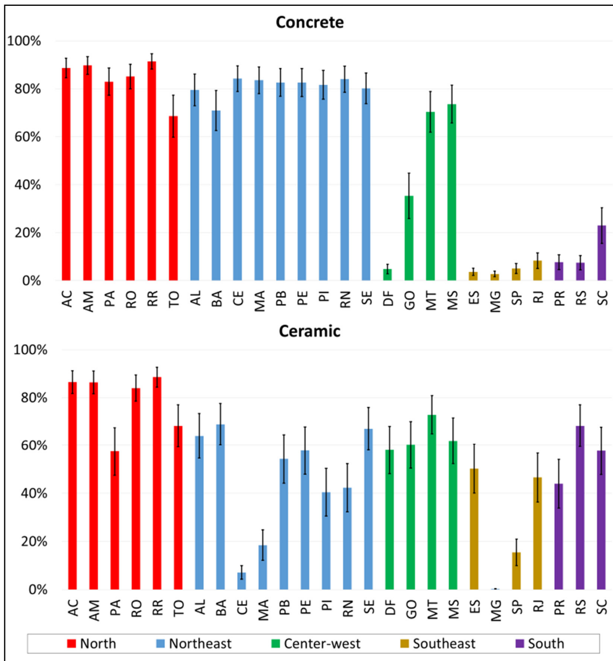
Figure 9. Percentage of the transportation stage in the Human Health impact. The error bars represent the standard deviation due to transportation scenarios.
