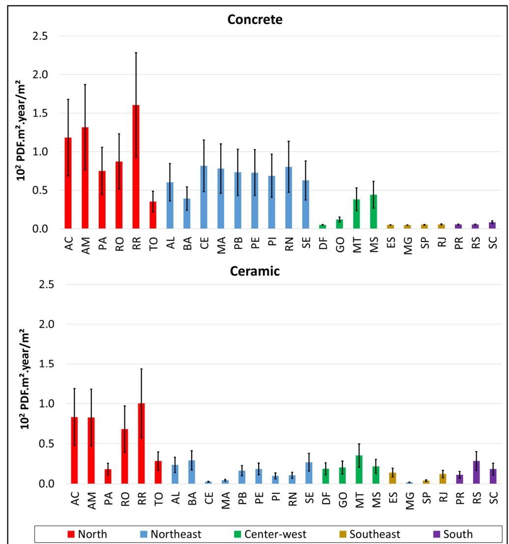
Figure 5. Total Ecosystem Quality impact. The error bars represent the standard deviation due to transportation scenarios.
