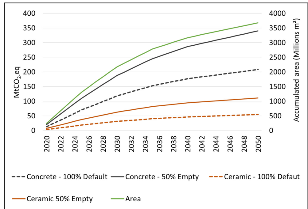
Figure 12. CO 2 -eq emissions considering the housing deficit projection; 100% Default—represents that the truck is loaded with 100% of its capacity and returns full; 50% empty—represents that the truck is loaded with 50% of its capacity and returns empty.
