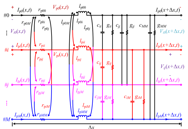
FIGURE 2. An improved MTL representation of an electrically small section \Delta x for an (M + 1) -conductor MTLs in time domain.
