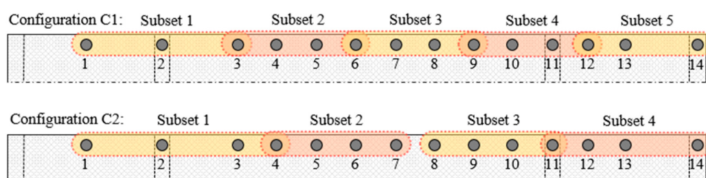
Figure 9. S101 bridge: Sensor subset configurations.
