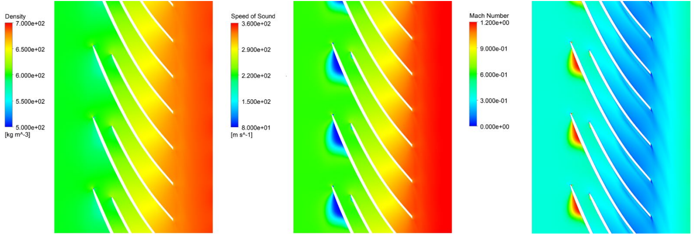
FIGURE 9: DISTRIBUTIONS OF DENSITY (LEFT), SPEED OF SOUND (CENTRE), AND RELATIVE MACH NUMBER (RIGHT) ON THE BLADE-TO-BLADE SURFACE AT 90% SPAN FOR LOW-TEMPERATURE INTAKE CONDITION
