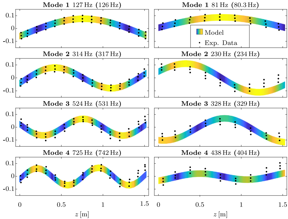
Fig. 7. The shapes of the first four (damped) bending modes in y direction. As the beam is almost symmetric, the modal shapes in x direction are very similar. The bending modes are shown for elastic (left) and bearing (right) supports. The deformation field is normalized for illustration purposes. The experimental values are in brackets.
