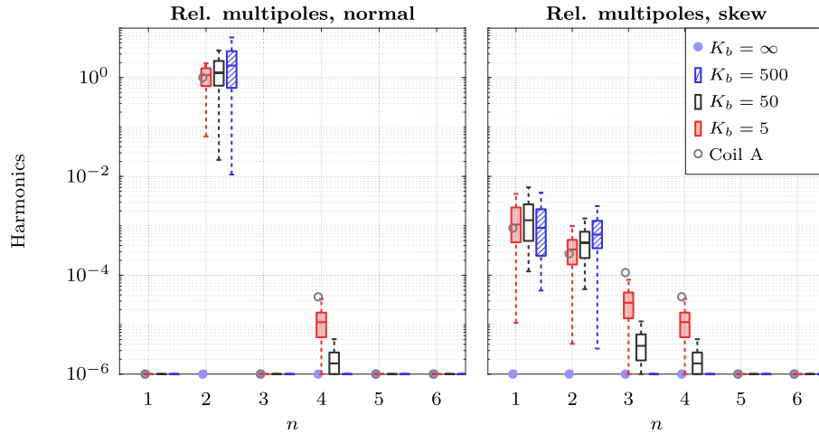
Fig. 10. Simulated measurement of an ideal quadrupole field, using a shaft under gravity and vibrations of the bearing at z = 1.52 m of 50 \mu\text{m} at \pi/4 . Spurious field multipoles as a function of the bucking ratio.
