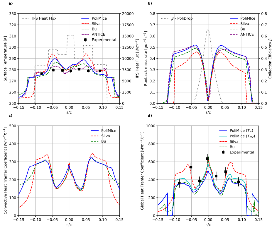
Figure 12: Results for the testcase 67B compared with experimental results from [4] and previous simulations presented in [20] [13]. In figure a) , the temperature at the surface of the airfoil is depicted. Figure b) shows the average runback water mass flowing at the surface of the airfoil. In figure c) , the convective heat transfer coefficient obtained is presented. In figure d) the overall heat transfer coefficient is shown.
