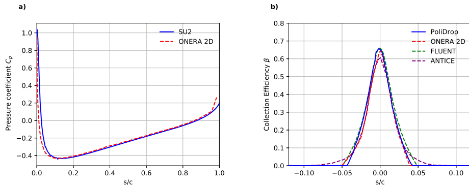
Figure 9: a) Computed pressure coefficient for the test case 67A and 67B obtained by means of SU2 and by Silva et al. [20] using the ONERA software. b) Water collection efficiency on the surface of the airfoil computed with PoliDrop [24] and by Silva et al. [20] by means of the ONERA software, Bu et al. [13] using FLUENT and by Al-Kalil et al. using the code ANTICE. [4]
