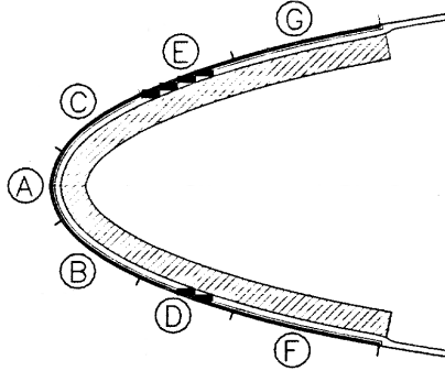
Figure 7: Airfoil leading edge and heated zones. [4]
