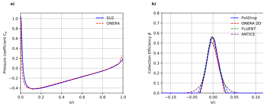
Figure 8: a) Computed pressure coefficient for the test case 22A obtained by means of SU2 and by Silva et al. [20] using the ONERA software. b) Water collection efficiency on the surface of the airfoil computed with PoliDrop [24] and by Silva et al. [20] by means of the ONERA software, Bu et al. [13] using FLUENT and by Al-Kalil et al. using the code ANTICE. [4]
