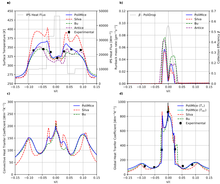
Figure 10: Results for the test case 22A compared with experimental results from [4] and previous simulations presented in [20] [13]. In figure a ), the temperature at the surface of the airfoil is depicted. Figure b ) shows the average runback water mass flowing at the surface of the airfoil. In figure c ), the convective heat transfer coefficient obtained is presented. In picture d ) the overall heat transfer coefficient is shown.
