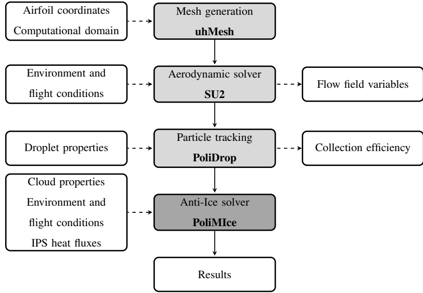
Figure 1: Flowchart of the PoliMICE framework for an anti-ice simulation.
