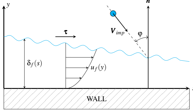
Figure 4: Water film detail. The parabolic velocity profile in the liquid film is highlighted along with the two driving forces: the wall shear stress \tau and the momentum per unit area from incoming water droplets
