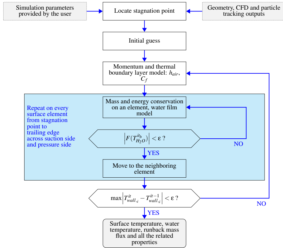
Figure 6: Flowchart of the numerical implementation of the model
