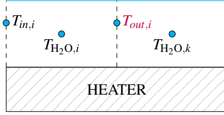
Figure 5: Interpolation points used in the computation of T_{out} of the i^{th} control volume: the temperature of the incoming water T_{in,i} , the water temperature in the control volume T_{H_2O,i} and the water temperature in the next control volume T_{H_2O,k} , according to the flow direction of the liquid film.
