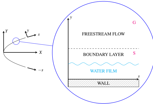
Figure 2: Airfoil reference system with a detail of the different zones of the physical problem. Region S is the region just above the liquid film which contains saturated vapor in equilibrium with the liquid phase. Region G represents the flow outside of the boundary layer where the vapor concentration is smaller
