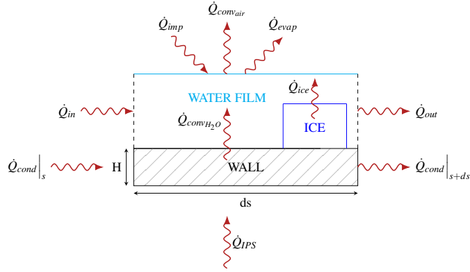
Figure 3: Contributions to energy conservation in a finite volume
