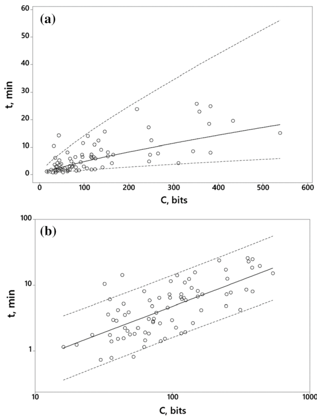
Fig. 1 Machining time as a function of complexity: a linear scale; b log–log scale
