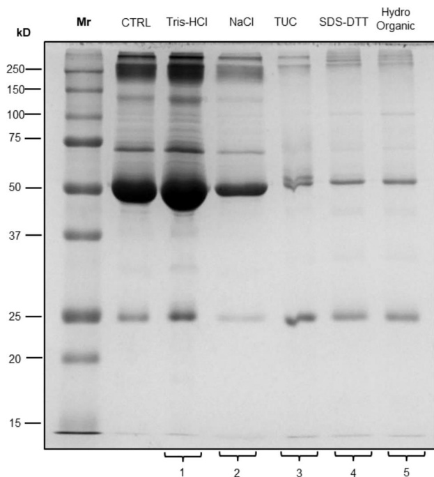
Fig. 2. SDS-PAGE containing protein profiles of different eluates: Tris-HCl (6 \mu l), NaCl (6 \mu l), TUC (3 \mu l), SDS-DTT (3 \mu l) and Hydro Organic (6 \mu l). All eluates were collected after incubation of 60 \mu l MWCNT-PEG5k with 1.94 mL human plasma at 37 °C. CTRL: 0.25 \mu l of human plasma (untreated sample).
