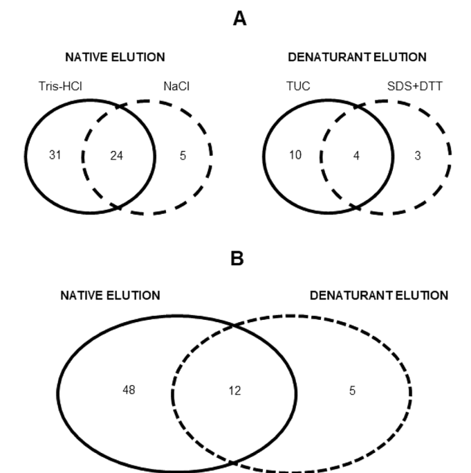
Fig. 4. Comparison native elution vs denaturant elution. (A) Venn diagrams highlighted all proteins eluted in native (Tris-HCl, NaCl) and denaturant (TUC, SDS-DTT and Hydro Organic) conditions, respectively. (B) Venn diagram compared proteins released in native and denaturant conditions.
