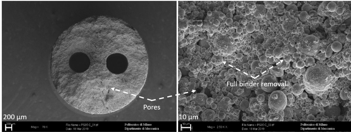
Fig. 7. SEM image of the bi-lumen tube cross-section at PS state.
