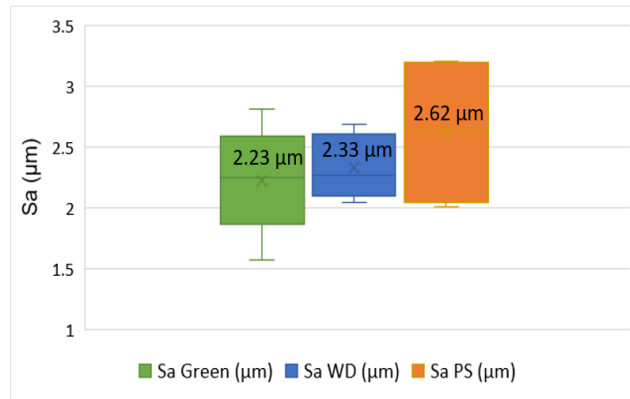
Fig. 4. Sa variation with respect to WD and PS.
