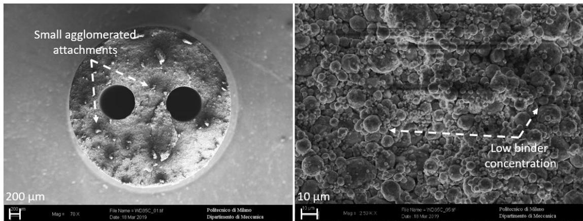
Fig. 6. SEM image of the bi-lumen tube cross-section at WD state.
