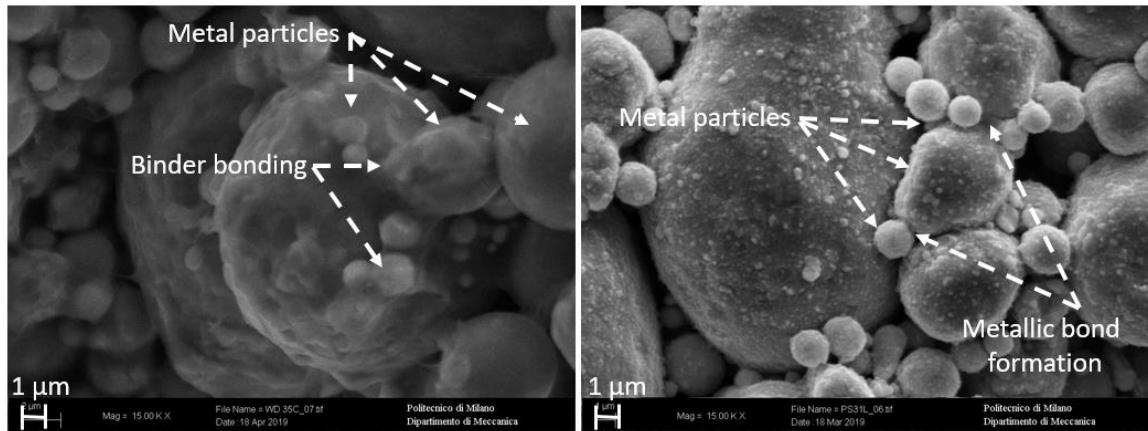
Fig. 8. SEM images of the metallic particle bonding at WD (left) and PS (right) states.
