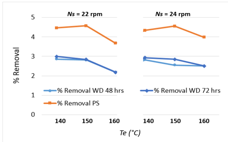
Fig. 3. % Removal of binder with respect to WD and PS.
