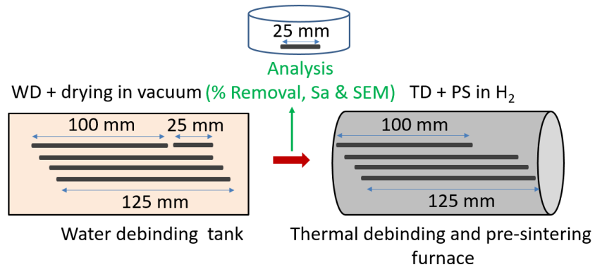
Fig. 2. The methodology used for WD and TD/PS.
