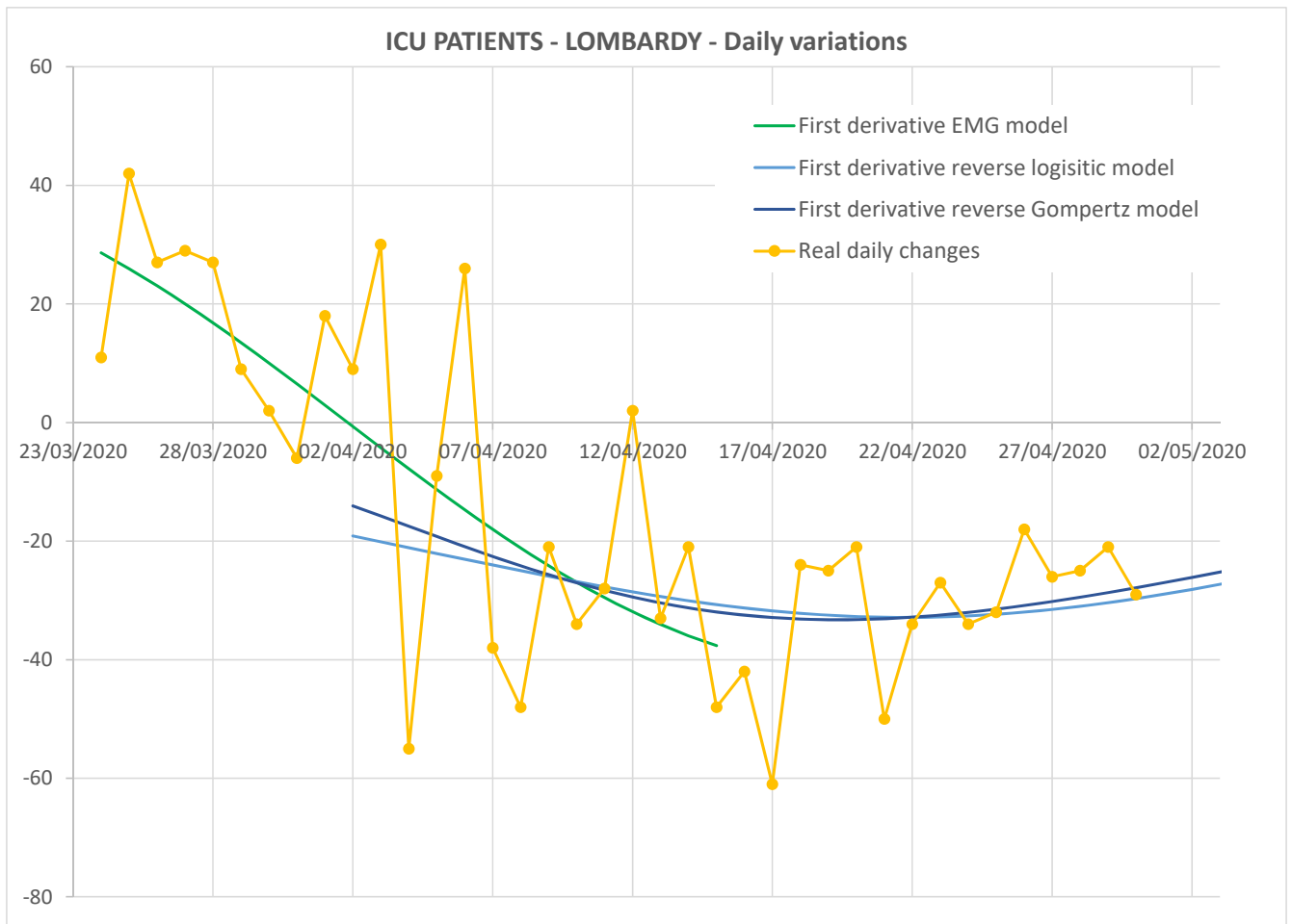
Figure 5: Daily variations of ICU patients in Lombardy. The lines show the first derivatives of the EMG, logistic, and Gompertz models.
