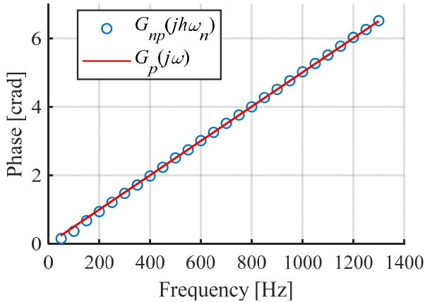
Fig. 6. Phase response: nonparametric and parametric inverse FRFs.
