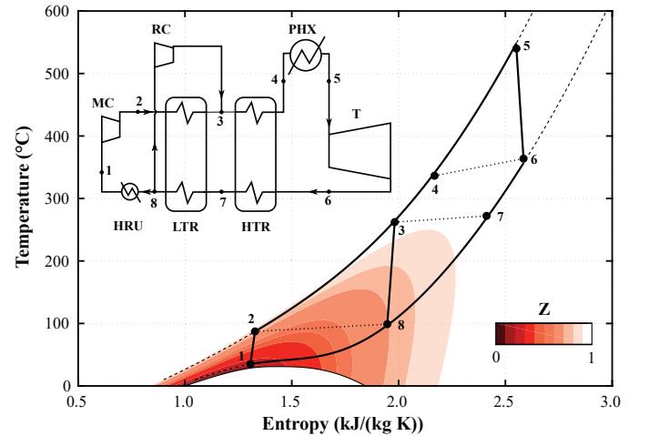
FIGURE 1: Recompression sCO 2 cycle layout and corresponding thermodynamic transformations on T-s plane. MC: Main compressor; RC: Recirculator; PHX: Primary Heat Exchanger; T: Turbine; HTR: High-Temperature Recuperator; LTR: Low-Temperature Recuperator; HRU: Heat Rejection Unit. A map of the compressibility factor Z = Pv/RT is superposed.
