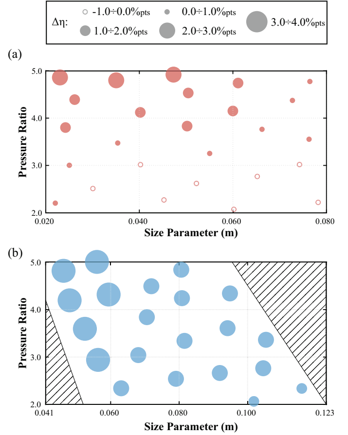
FIGURE 8: Efficiency deviation \Delta\eta between dedicated optimizations of two-stage machines and predicted efficiencies by single-stage correlations for compressors (a) and turbines (b).
