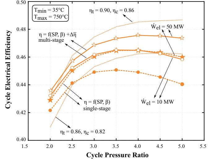
FIGURE 9: Cycle efficiency \eta_{el} evolution as a function of the cycle pressure ratio P_{max}/P_{min} for two installed power capacities by employing single- and multi-stage turbomachinery.
