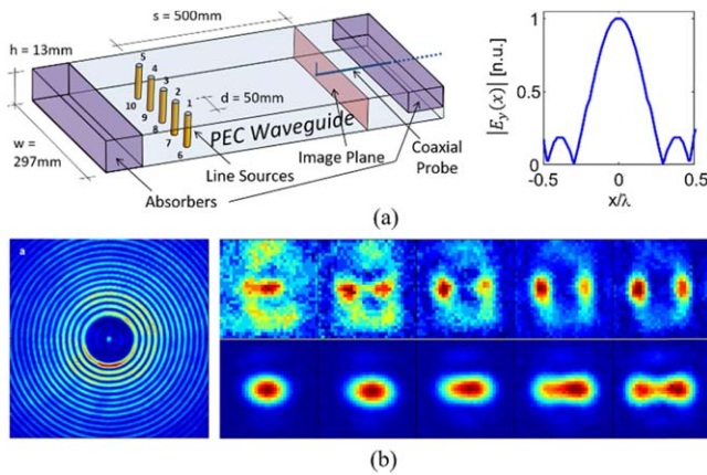
Figure 13. Examples of antenna-based approach to spatial super-oscillation design. (a) 1D subwavelength hotspot in a waveguide. Schematic (left) and the simulated subwavelength focus (right). © IEEE. Reprinted, with permission, from [89]. (b) Experimental measurements using the optical super-microscope (OSM). The OSM’s point-spread function (left) and the resolving of two apertures (right: top row = OSM, bottom row = diffraction limit). Reprinted by permission from Springer Nature: Scientific Reports [46], (2013).
