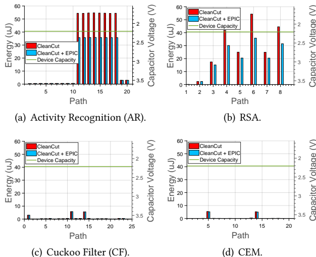
Figure 12. CleanCut results. Using EPIC with CleanCut, false positives are avoided when looking for non-termination bugs.
