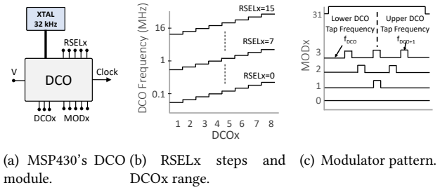
Figure 4. Impact of DCO parameters on clock.
