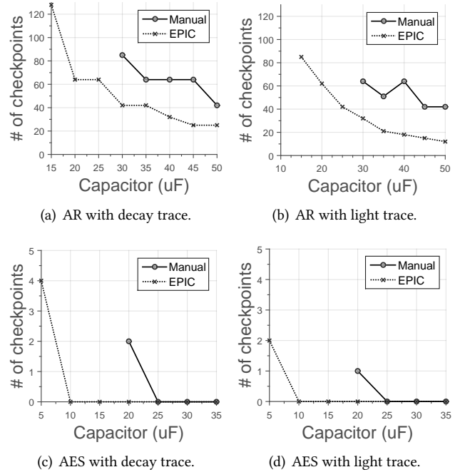
Figure 11. HarvOS results. The benefits of using EPIC within HarvOS apply across different capacitor sizes.
