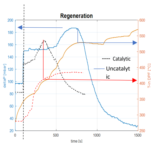
Figure 1. \Delta P (dotted black curve) and inlet Temperature ( T_{\text{in}} ) (dotted red curve) vs regeneration time for 30%wt \text{CuFe}_2\text{O}_4 catalytic filter and the uncatalytic DPF (continuous lines).
