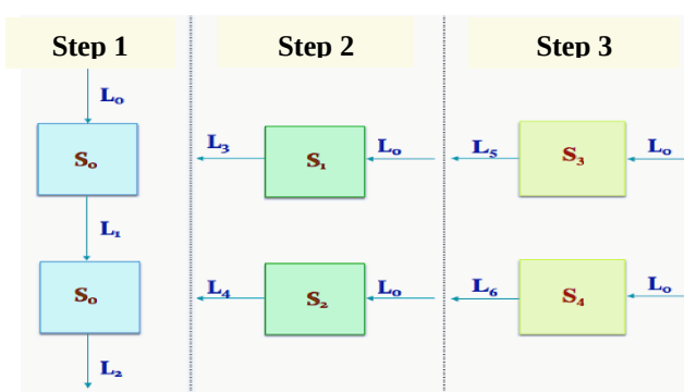
Fig.2: Cross-flow extraction scheme [3 steps - 2 batches]
