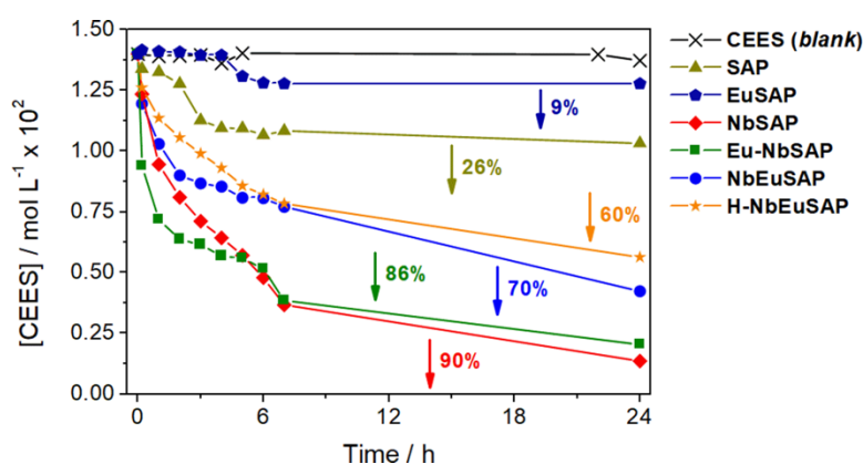
Figure 1. Oxidative abatement of CEES with hydrogen peroxide over different saponite samples containing Eu(III) and/or Nb(V) sites. Reaction conditions: 14 mM CEES, 70 mM 30% aq. H 2 O 2 , phosphate buffer solution (PBS, 10 mM, pH = 7), 20 mg catalyst, 298 K.
