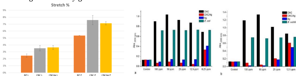
Fig. 2. (Left) Relative maximum elongation for not treated paper, CNC and CNC/nAg treated paper samples (L = longitudinal, P = perpendicular). (Right) (a) Growth of E.coli and (b) B.subtilis in the presence of CNC, a mix of CNC/nAg and nAg alone at different concentrations for MIC determination
