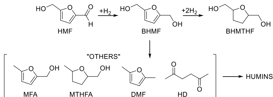
Scheme 1. Reaction network proposed for the hydrogenation and hydrogenolysis of HMF in water. (MFA: 5-methylfurfuryl alcohol; MTHFA: 5-methyltetrahydrofurfuryl alcohol; DMF: 2,5-dimethylfuran; HD: 2,5-hexanedione)
