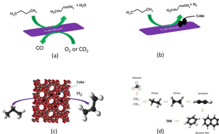
Four new approaches using advanced catalysts addressed in BIZEOLCAT a) oxidative BDH and b) non oxidative BDH c) PDH and d) Aromatization of methane with improved reactor technologies.
