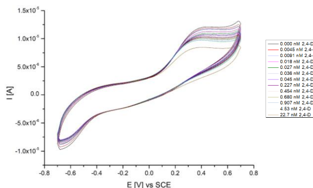
Figure 1. Voltammograms ( 0.05 \text{ V s}^{-1} ) recorded in Tris buffer containing 3 mM AAP and different amounts of 2,4-D herbicide.
