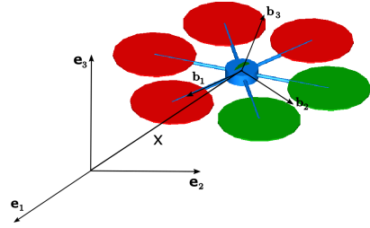
Fig. 1 Example of a multirotor UAV and definition of the frames.
