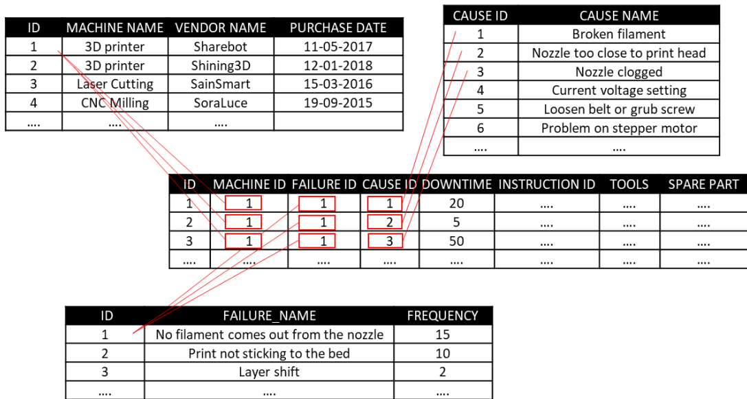
Figure 6: The link of asset information in a relational database.
