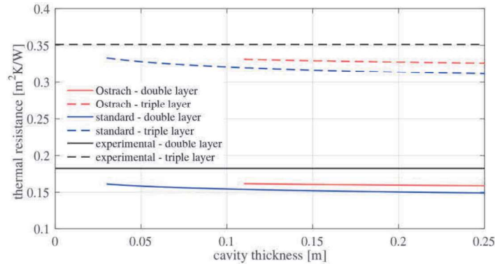
Figure 5: comparison between the experimental thermal resistances, obtained for both Box 1 and Box 2, and the results achieved using correlations from literature for vertical rectangular cavities.
